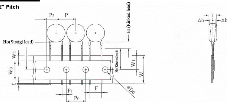
1.0" Pitch
