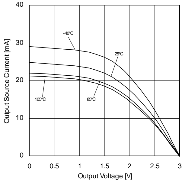
Figure 56. Output Source Current vs Output Voltage (VDD=3V)
