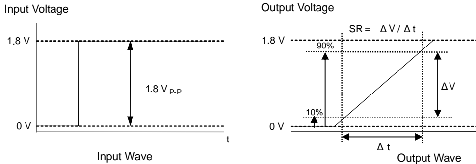
Figure 73. Slew Rate Input Output Wave
