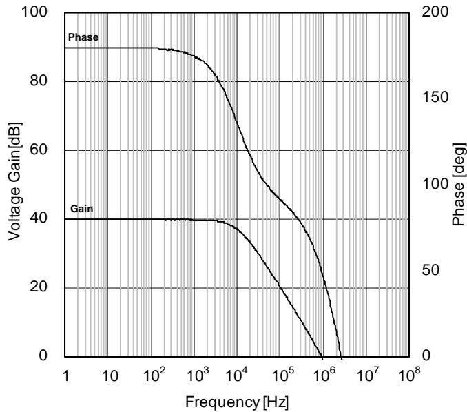
Figure 70. Voltage Gain • Phase vs Frequency
