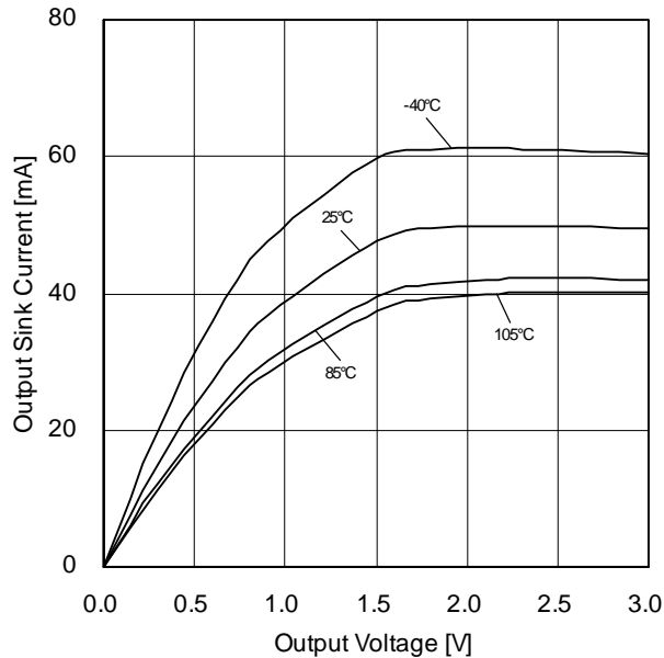
Figure 12. Output Sink Current vs Output Voltage (VDD=3V)
