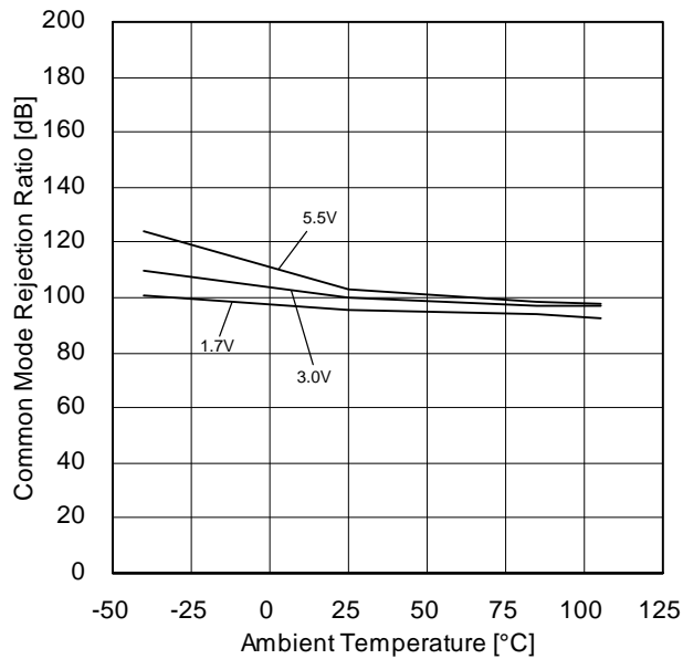
Figure 20. Common Mode Rejection Ratio vs Ambient Temperature
