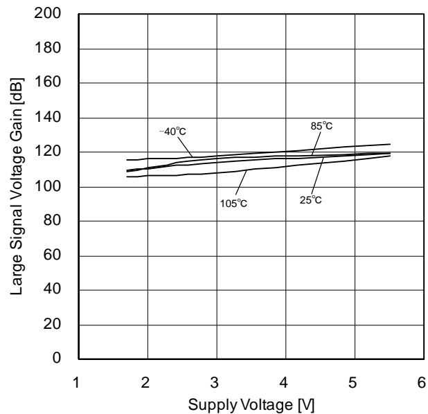
Figure 40. Large Signal Voltage Gain vs Supply Voltage
