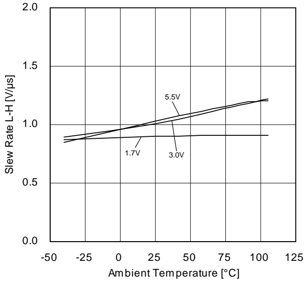
Figure 68. Slew Rate L-H vs Ambient Temperature
