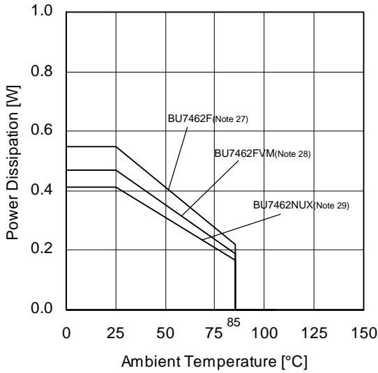
(e) BU7462xxx
