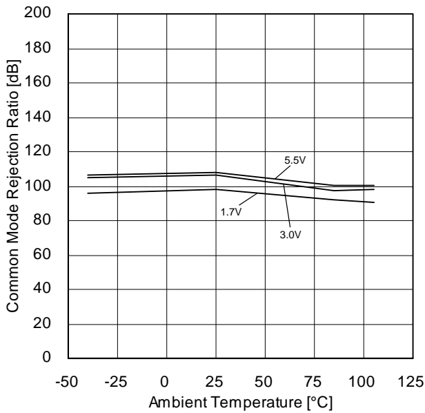
Figure 66. Common Mode Rejection Ratio vs Ambient Temperature
