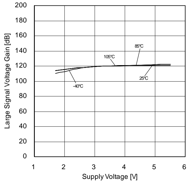
Figure 63. Large Signal Voltage Gain vs Supply Voltage
