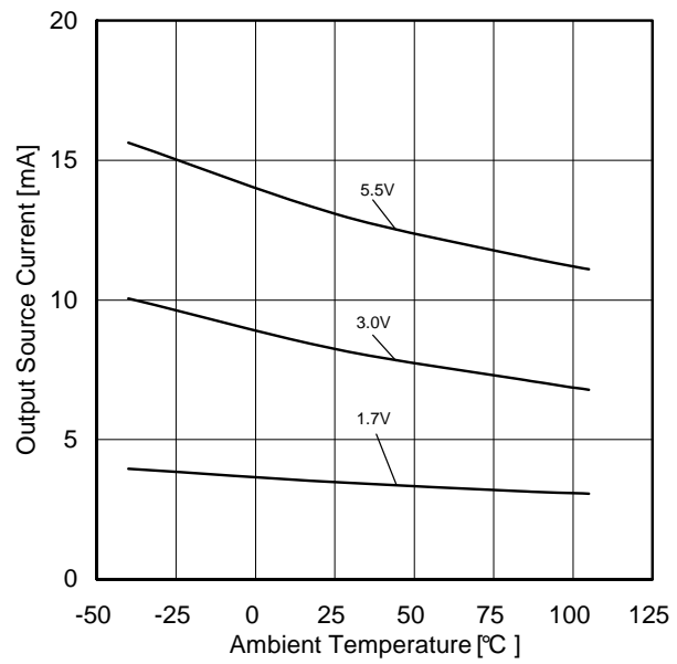
Figure 34. Output Source Current vs Ambient Temperature (OUT=VDD-0.4V)
