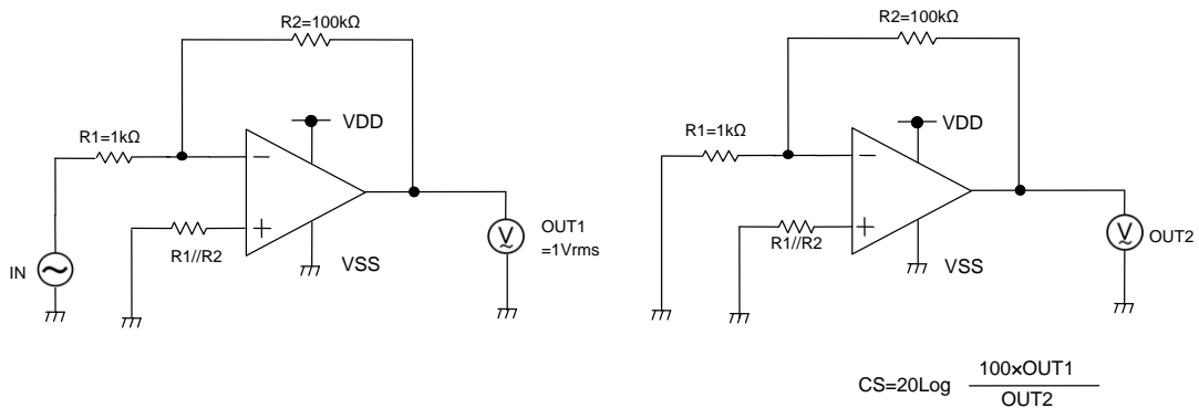
Figure 74. Test Circuit 3(Channel Separation)
