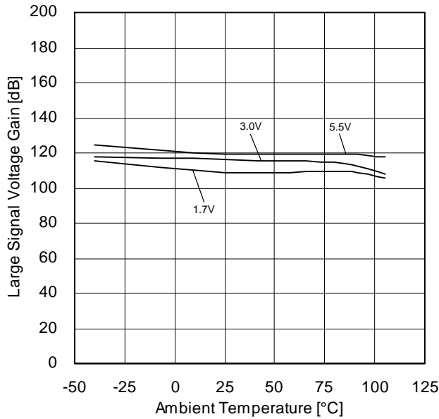
Figure 41. Large Signal Voltage Gain vs Ambient Temperature
