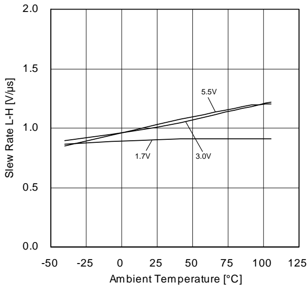
Figure 22. Slew Rate L-H vs Ambient Temperature
