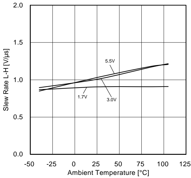
Figure 45. Slew Rate L-H vs Ambient Temperature
