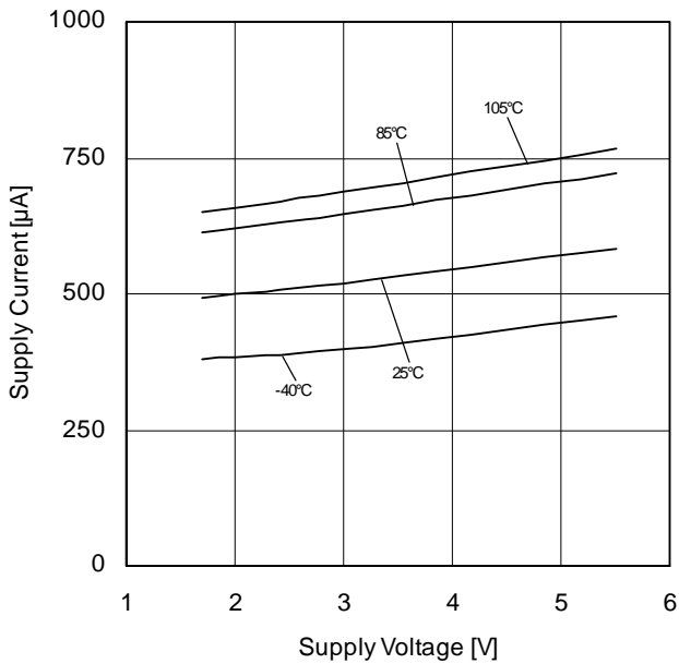
Figure 50. Supply Current vs Supply Voltage
