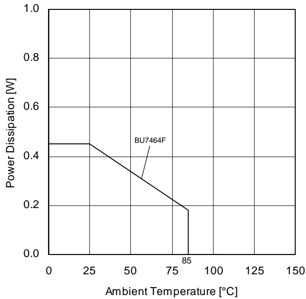
Figure 48. Power Dissipation vs Ambient Temperature Derating Curve
