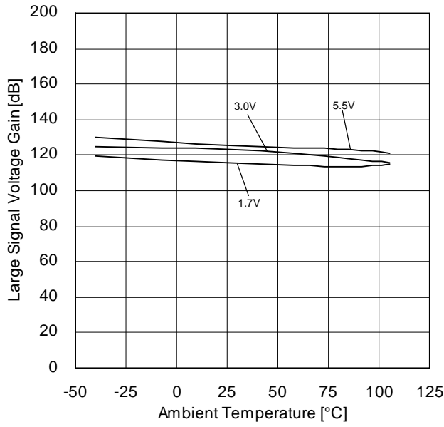
Figure 18. Large Signal Voltage Gain vs Ambient Temperature
