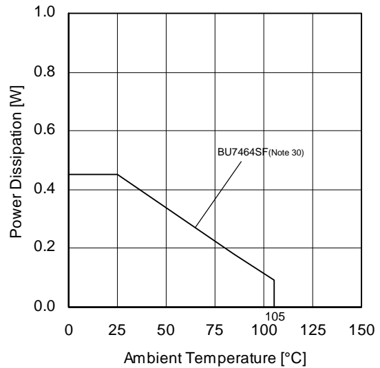
(h) BU7464SF
