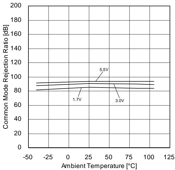
Figure 43. Common Mode Rejection Ratio vs Ambient Temperature
