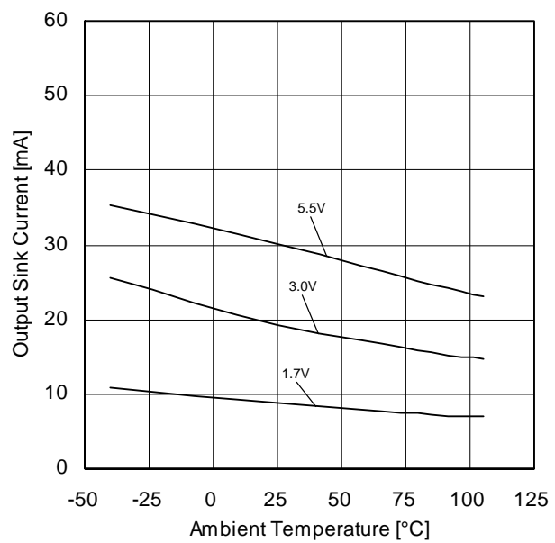
Figure 36. Output Sink Current vs Ambient Temperature (OUT=VSS+0.4V)
