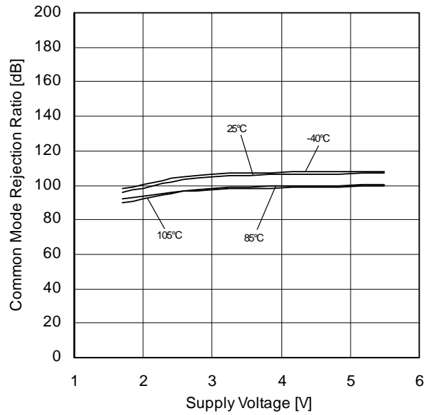
Figure 65. Common Mode Rejection Ratio vs Supply Voltage
