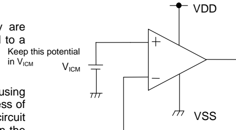
Figure 79. Example of Application Circuit for Unused Op-amp
