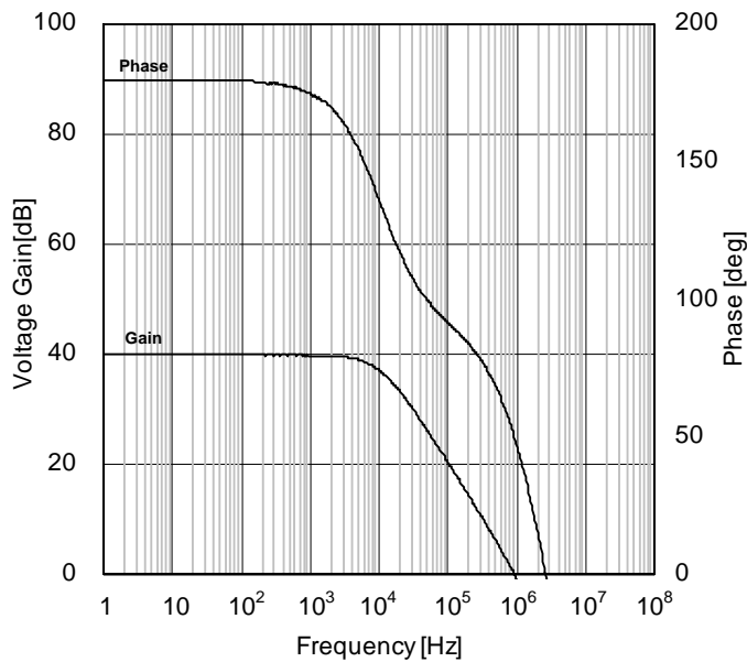
Figure 24. Voltage Gain · Phase vs Frequency
