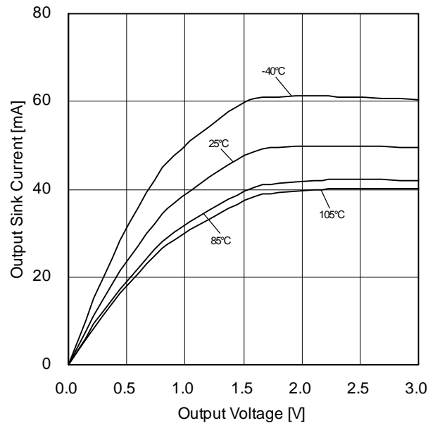
Figure 58. Output Sink Current vs Output Voltage (VDD=3V)
