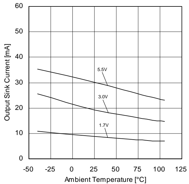
Figure 59. Output Sink Current vs Ambient Temperature (OUT=VSS+0.4V)
