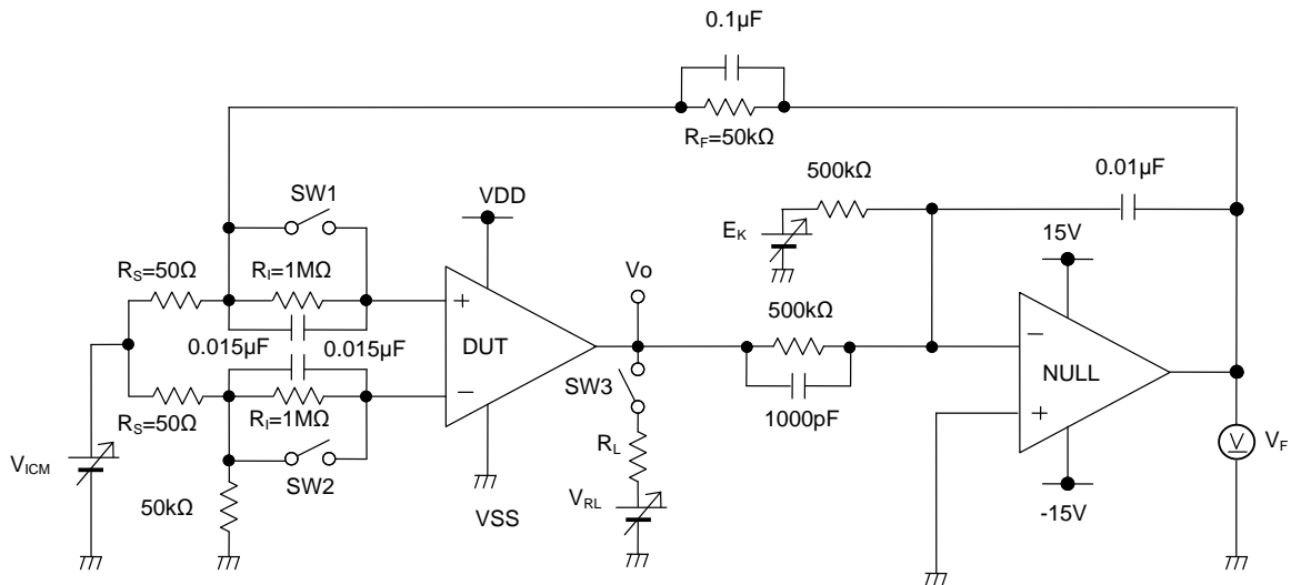
Figure 71. Test Circuit 1 (One Channel Only)
