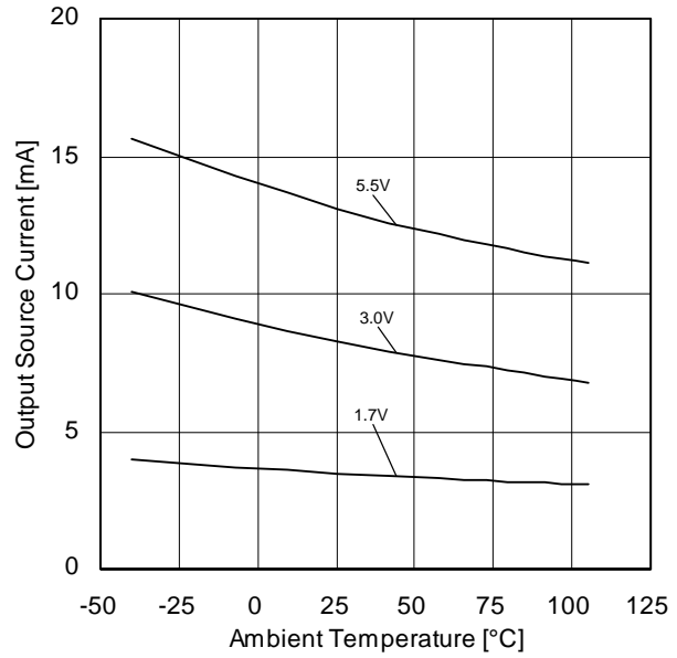
Figure 57. Output Source Current vs Ambient Temperature (OUT=VDD-0.4V)
