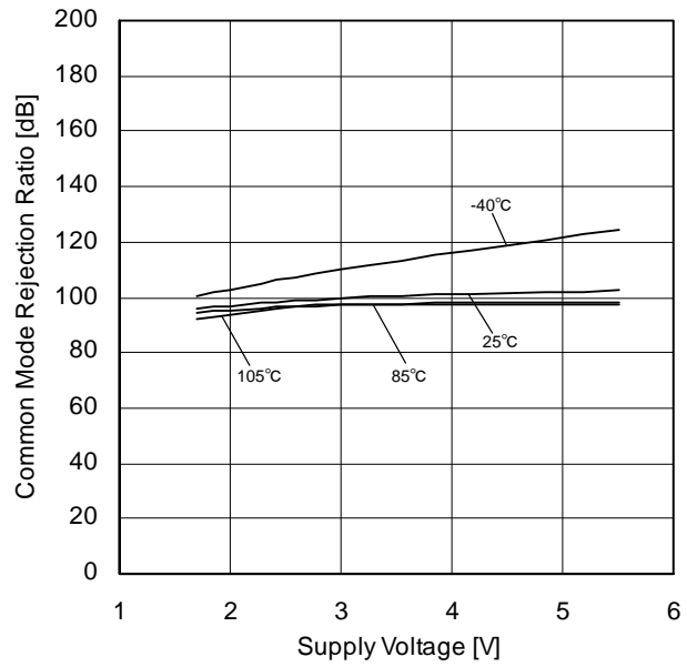
Figure 19. Common Mode Rejection Ratio vs Supply Voltage
