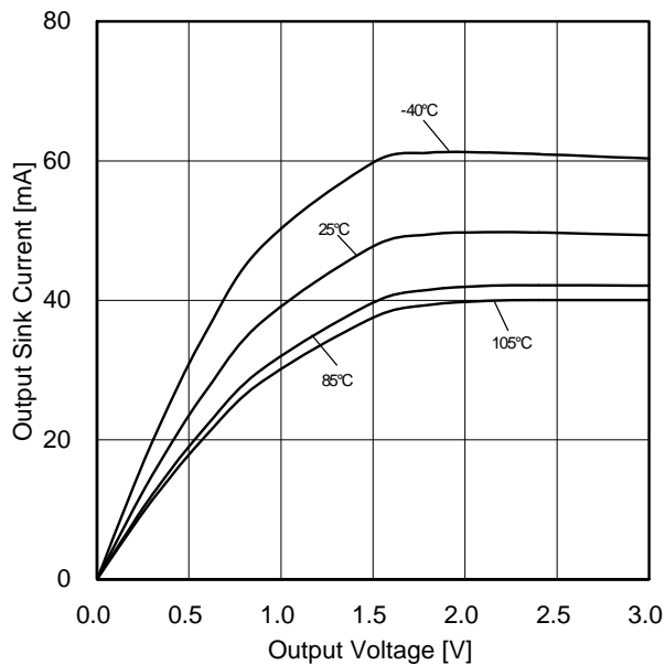
Figure 35. Output Sink Current vs Output Voltage (VDD=3V)
