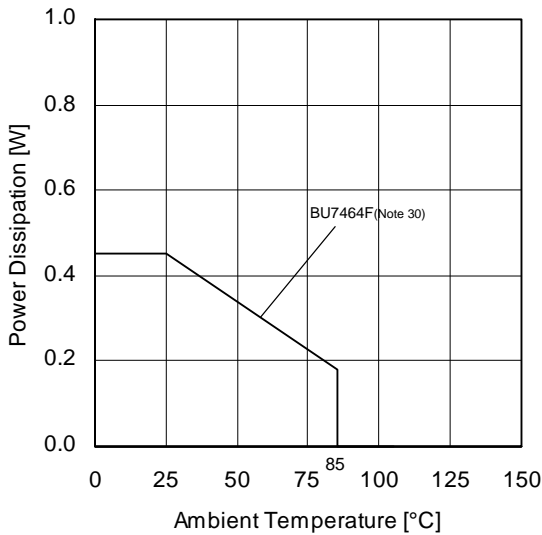
(g) BU7464F
