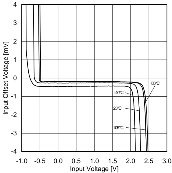
Figure 62. Input Offset Voltage vs Input Voltage ( V_{DD}=3V )
