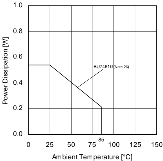
(c) BU7461G
