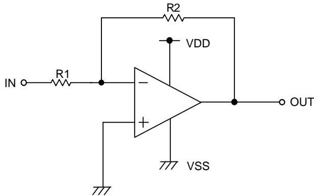
Figure 76. Inverting Amplifier Circuit
