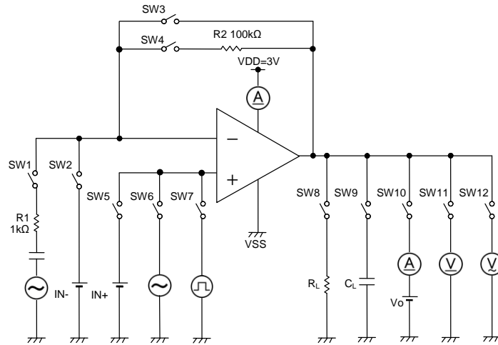
Figure 72. Test Circuit 2 (each channel)
