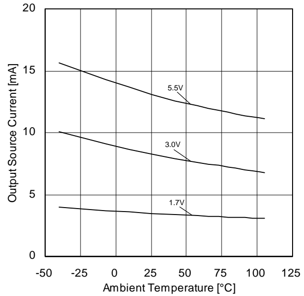
Figure 11. Output Source Current vs Ambient Temperature (OUT=VDD-0.4V)
