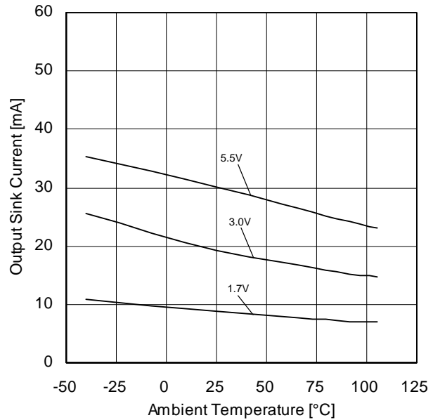
Figure 13. Output Sink Current vs Ambient Temperature (OUT=VSS+0.4V)
