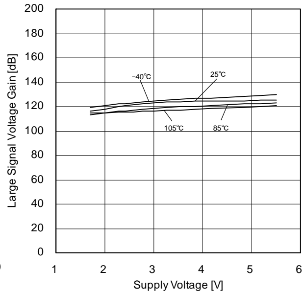
Figure 17. Large Signal Voltage Gain vs Supply Voltage
