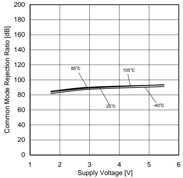
Figure 42. Common Mode Rejection Ratio vs Supply Voltage
