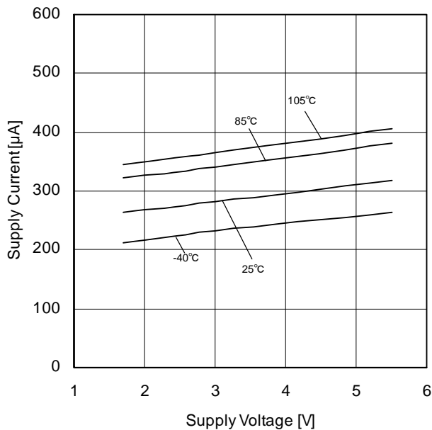
Figure 27. Supply Current vs Supply Voltage
