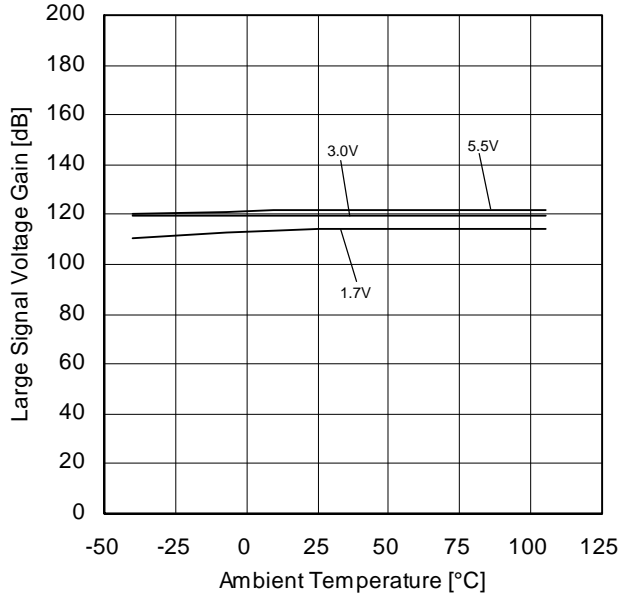
Figure 64. Large Signal Voltage Gain vs Ambient Temperature
