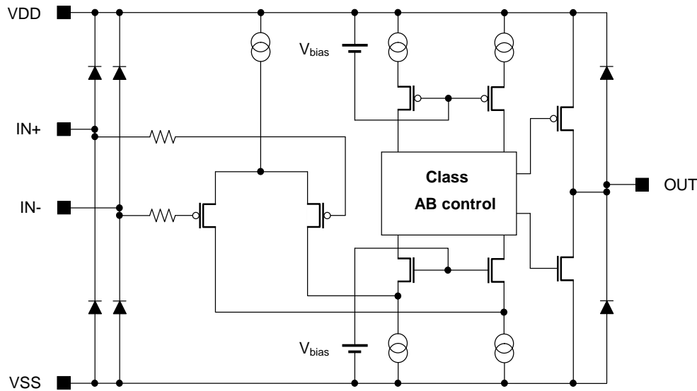
Figure 1. Simplified Schematic (1 channel only)
