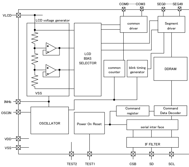
Fig.10 Block Diagram (BU9794AKV)
