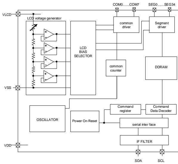
Fig.14 Block Diagram (BU97950KS2)
