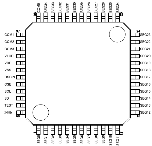
Fig.5 Pin Arrangement (BU9795AKV)
