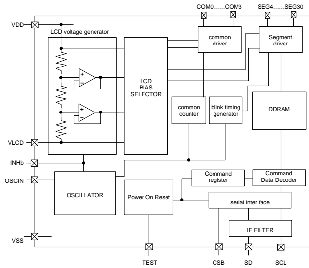
Fig.6 Block Diagram (BU9795AFV)
