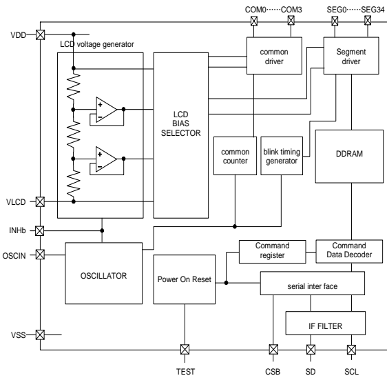
Fig.4 Block Diagram (BU9795AKV)
