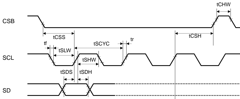
Fig.1 Interface Timing (BU9795AKV/FV/GUW)
