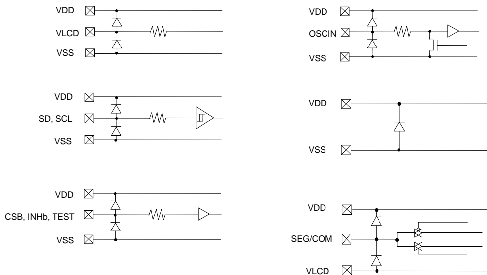
Fig.16 I/O equivalent circuit (BU9795AKV/FV/GUW)
