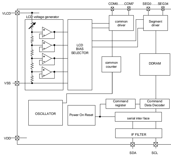
Fig.12 Block Diagram (BU97950FUV)
