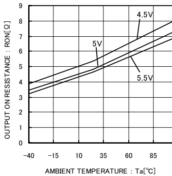
Fig.4 Output on resistance (Temperature characteristic @ IDD=20mA)
