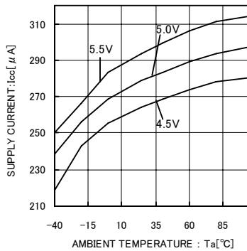
Fig.2 Circuit current (Temperature characteristic)
