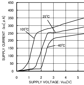
Fig.1 Circuit current (VCC characteristic)
