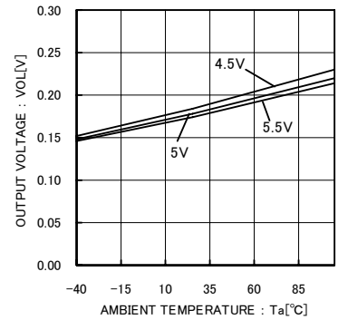
Fig.9 SEROUT low side voltage (Temperature characteristic @ ISO=4mA)
