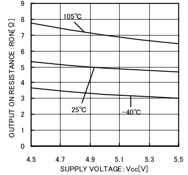
Fig.3 Output on resistance (VCC characteristic @ IDD=20mA)
