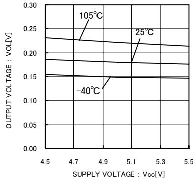
Fig.8 SEROUT low side voltage (VCC characteristic @ ISO=5mA)
