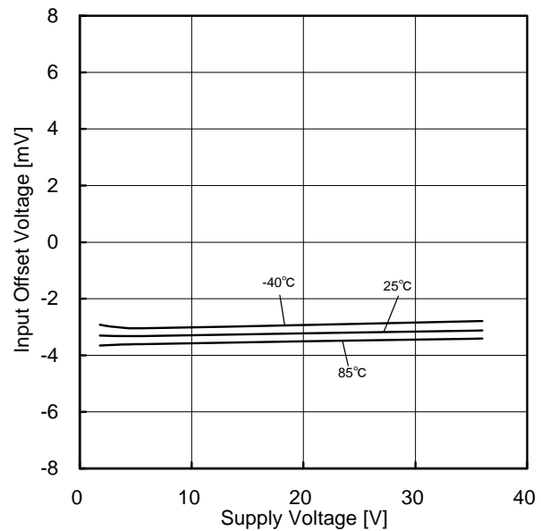
Figure 52. Input Offset Voltage vs Supply Voltage
