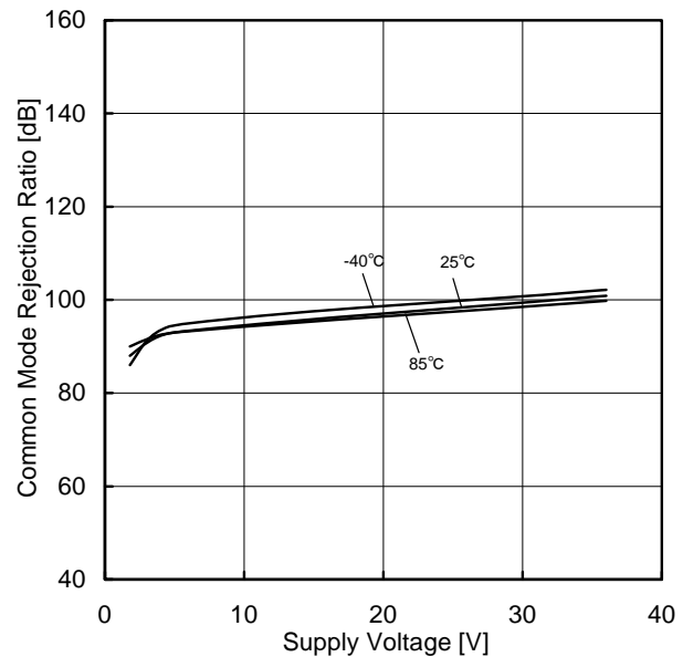
Figure 60. Common Mode Rejection Ratio vs Supply Voltage
