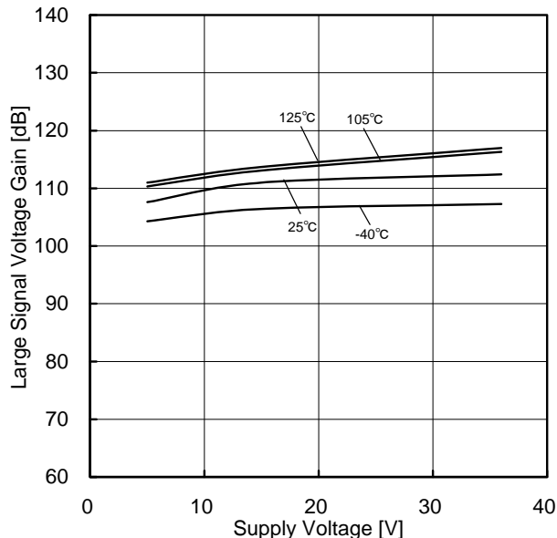
Figure 78. Large Signal Voltage Gain vs Supply Voltage
