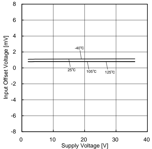
Figure 72. Input Offset Voltage vs Supply Voltage
