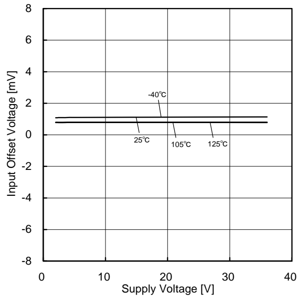
Figure 95. Input Offset Voltage vs Supply Voltage
