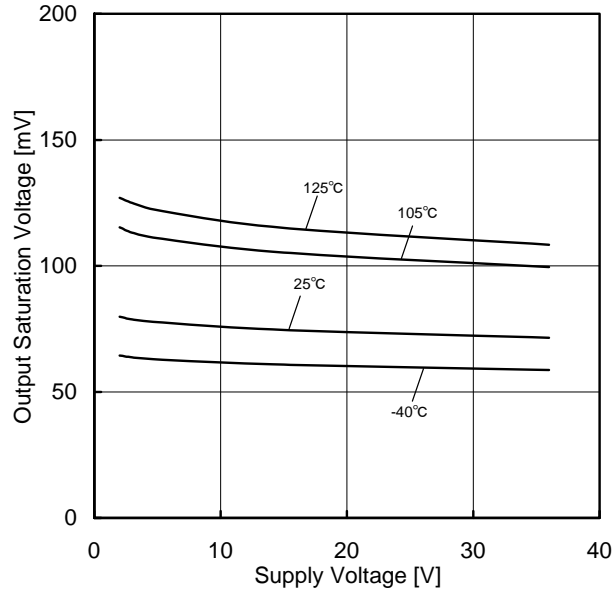
Figure 91. Output Saturation Voltage vs Supply Voltage ( I_{OL}=4mA )
