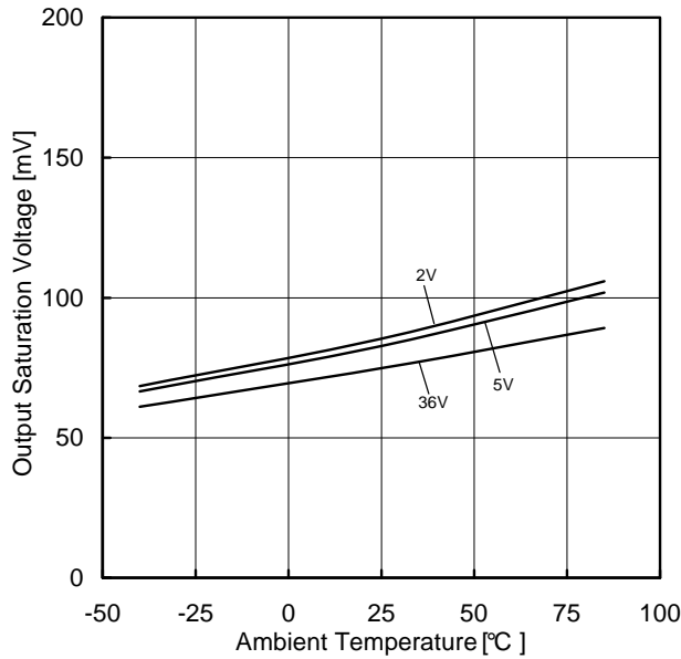
Figure 6. Output Saturation Voltage vs Ambient Temperature ( I_{OL}=4mA )
