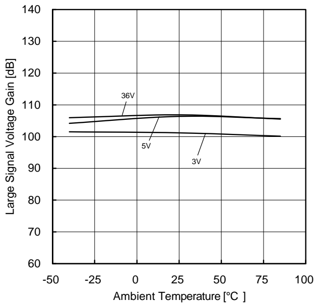
Figure 59. Large Signal Voltage Gain vs Ambient Temperature
