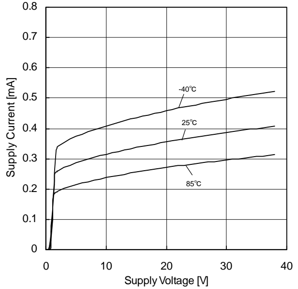
Figure 3. Supply Current vs Supply Voltage
