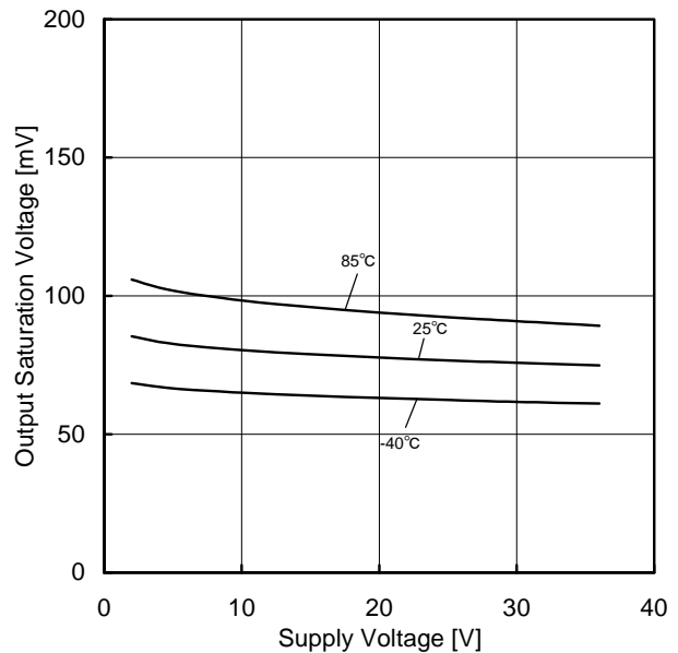
Figure 5. Output Saturation Voltage vs Supply Voltage ( I_{OL}=4mA )
