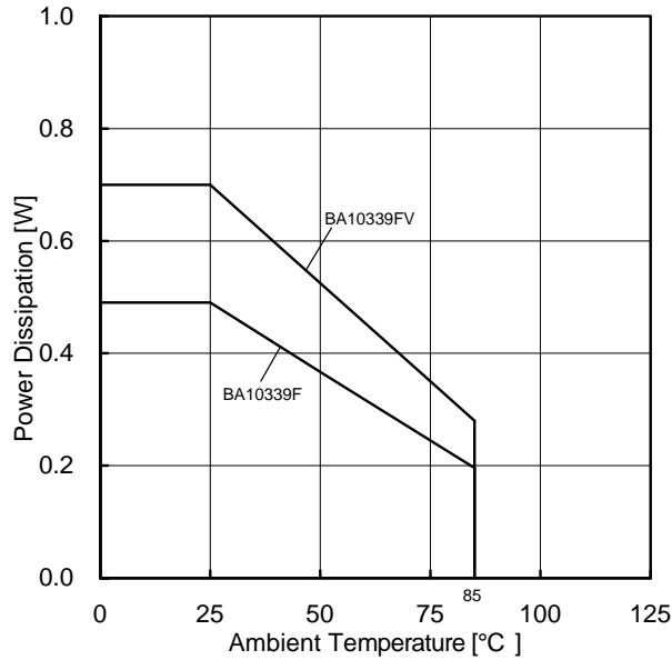
Figure 45. Power Dissipation vs Ambient Temperature (Derating Curve)
