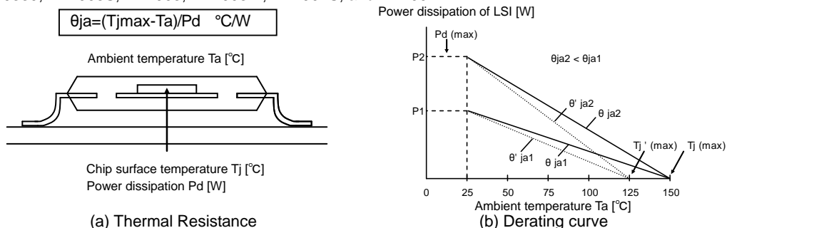
Figure 114. Thermal Resistance and Derating Curve
