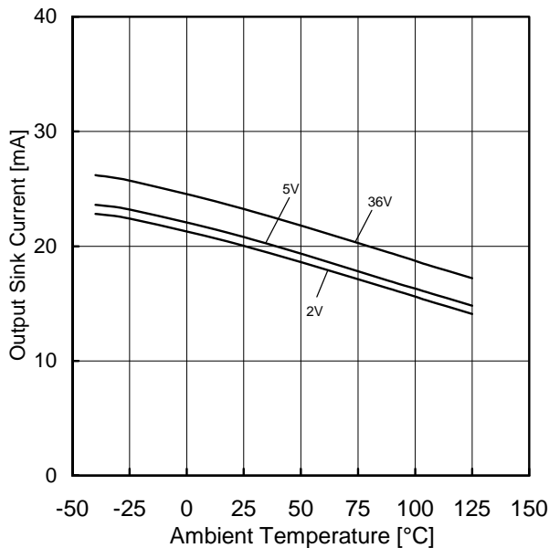
Figure 94. Output Sink Current vs Ambient Temperature ( OUT=1.5V )
