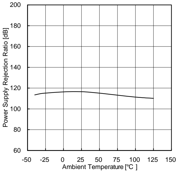
Figure 83. Power Supply Rejection Ratio vs Ambient Temperature
