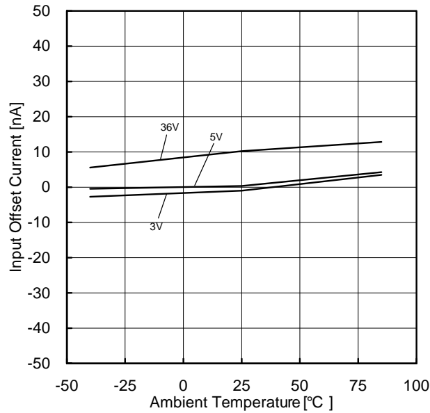
Figure 57. Input Offset Current vs Ambient Temperature
