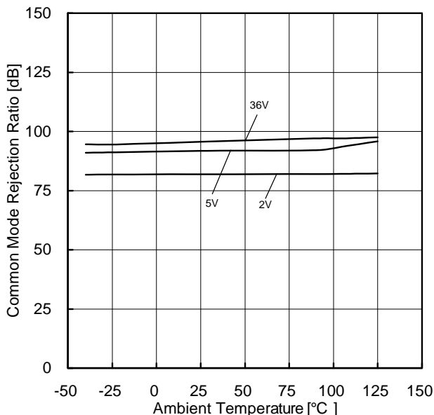
Figure 104. Common Mode Rejection Ratio vs Ambient Temperature
