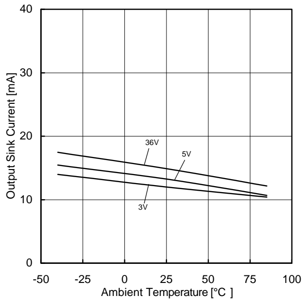
Figure 51. Output Sink Current vs Ambient Temperature ( OUT=1.5V )
