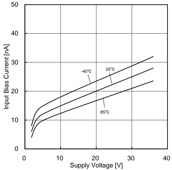
Figure 54. Input Bias Current vs Supply Voltage
