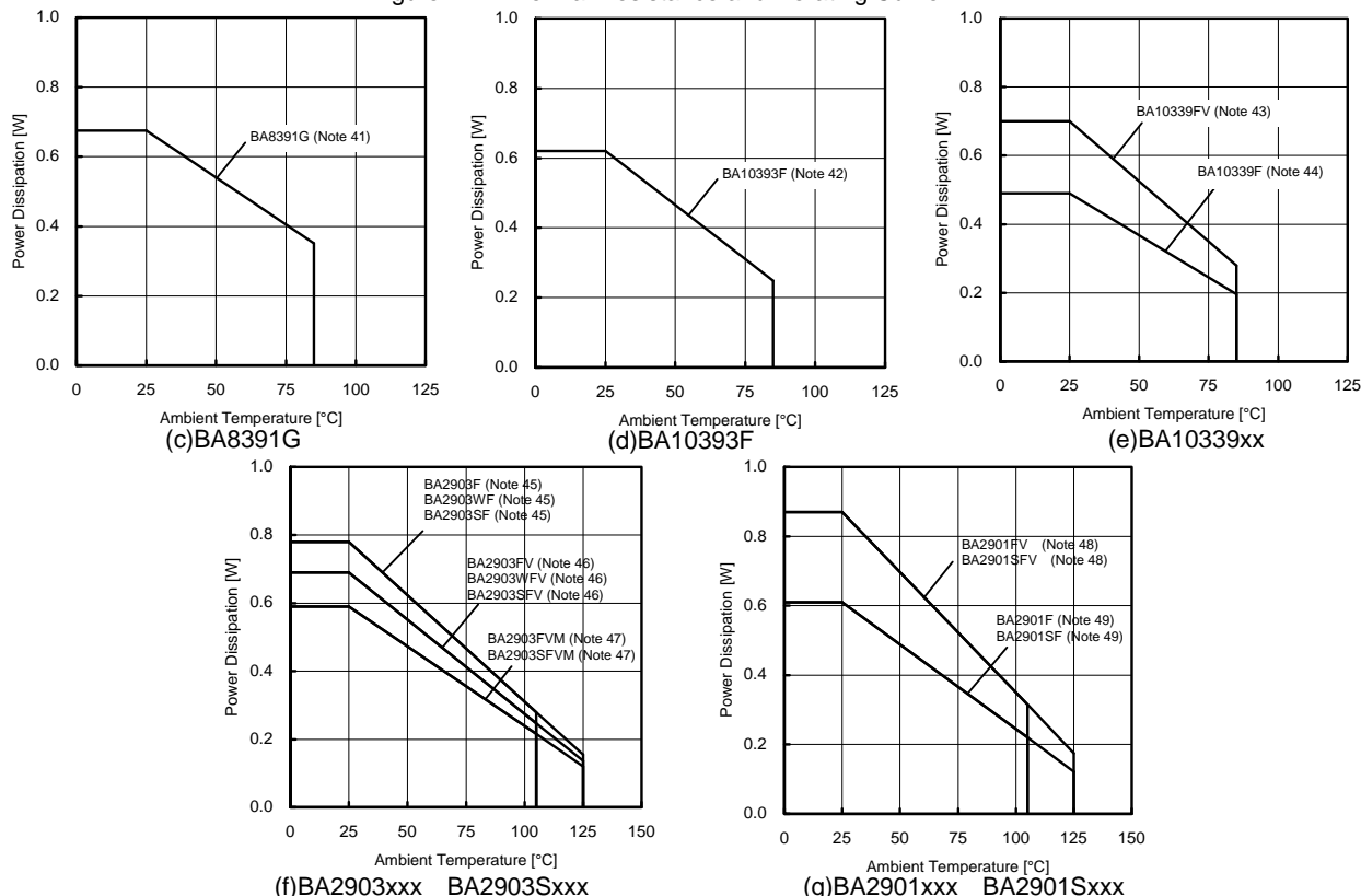
Figure 114. Thermal Resistance and Derating Curve
