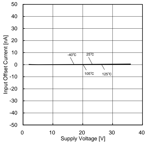
Figure 99. Input Offset Current vs Supply Voltage
