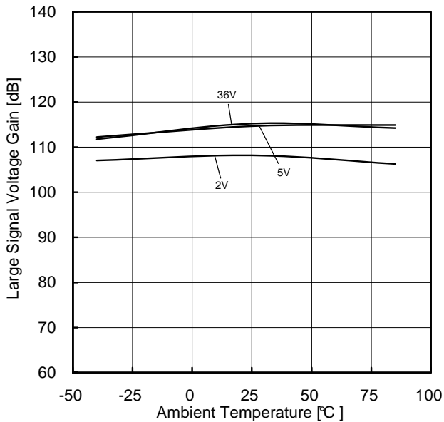
Figure 39. Large Signal Voltage Gain vs Ambient Temperature
