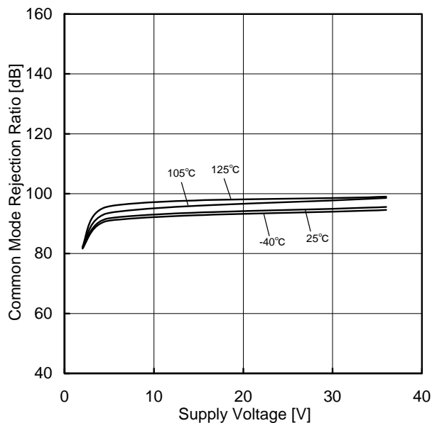
Figure 80. Common Mode Rejection Ratio vs Supply Voltage
