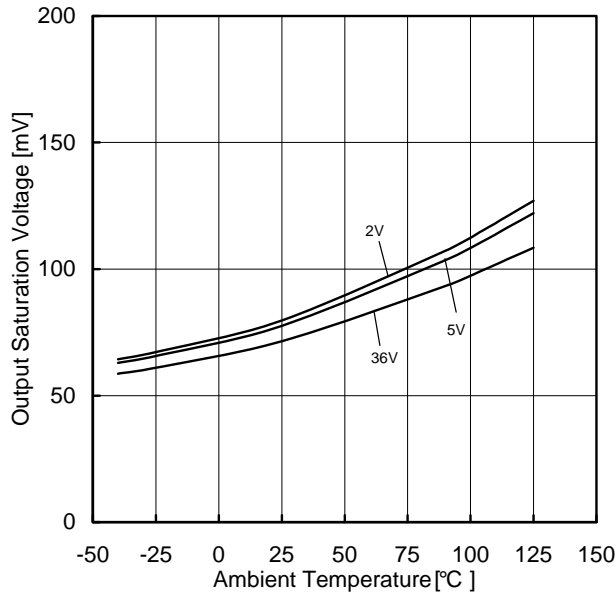
Figure 92. Output Saturation Voltage vs Ambient Temperature ( I_{OL}=4mA )
