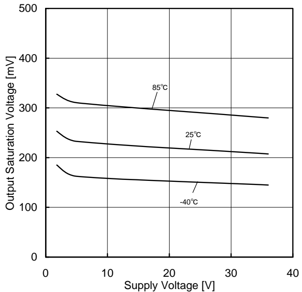
Figure 48. Output Saturation Voltage vs Supply Voltage ( I_{OL}=4mA )
