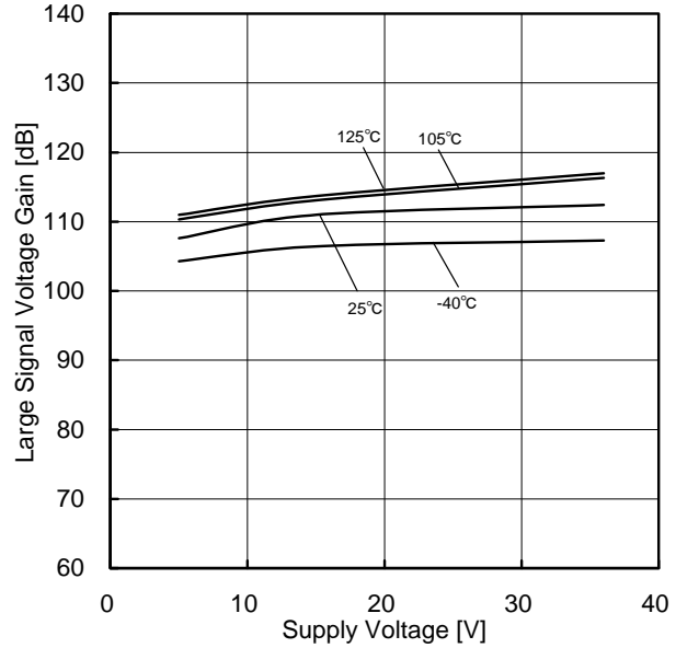
Figure 101. Large Signal Voltage Gain vs Supply Voltage
