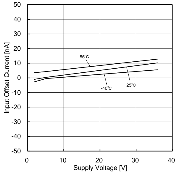
Figure 56. Input Offset Current vs Supply Voltage
