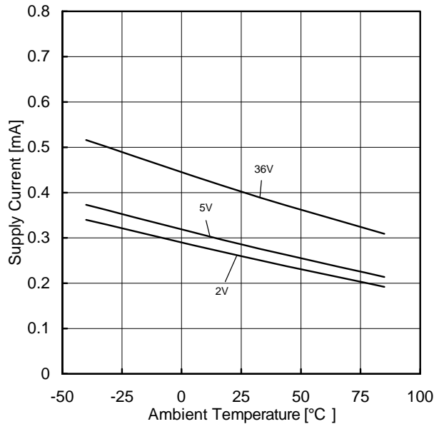
Figure 4. Supply Current vs Ambient Temperature
