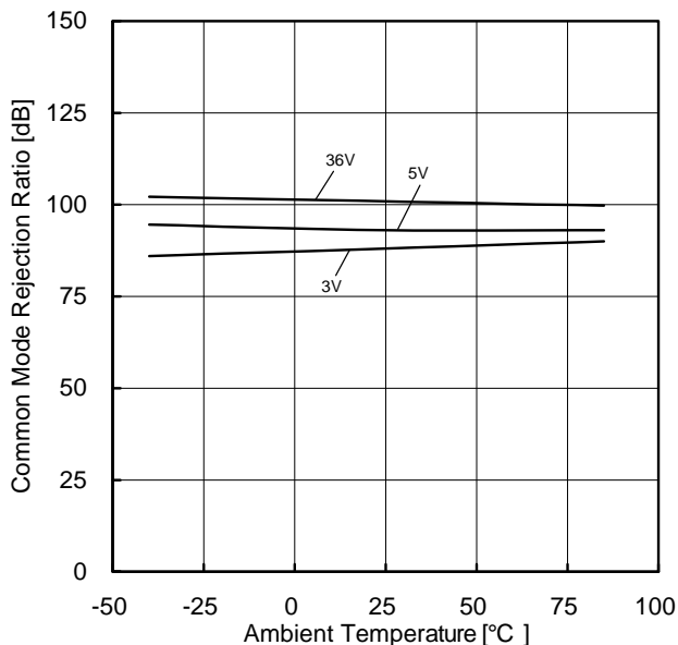
Figure 61. Common Mode Rejection Ratio vs Ambient Temperature
