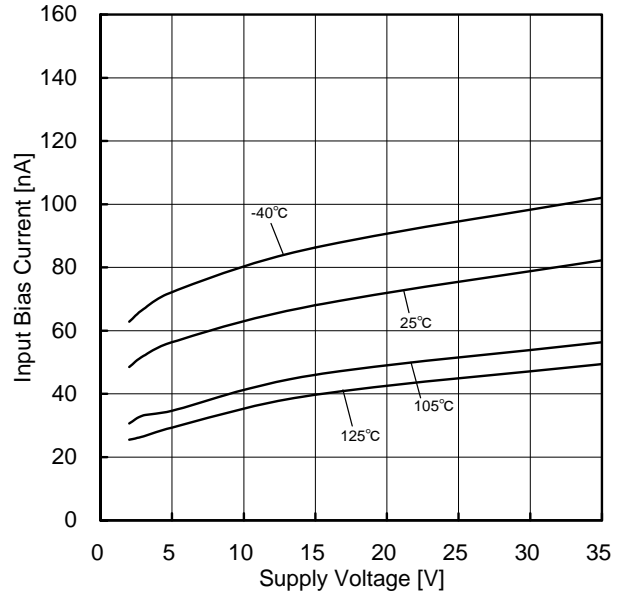
Figure 74. Input Bias Current vs Supply Voltage
