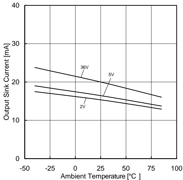
Figure 31. Output Sink Current vs Ambient Temperature (OUT=1.5V)
