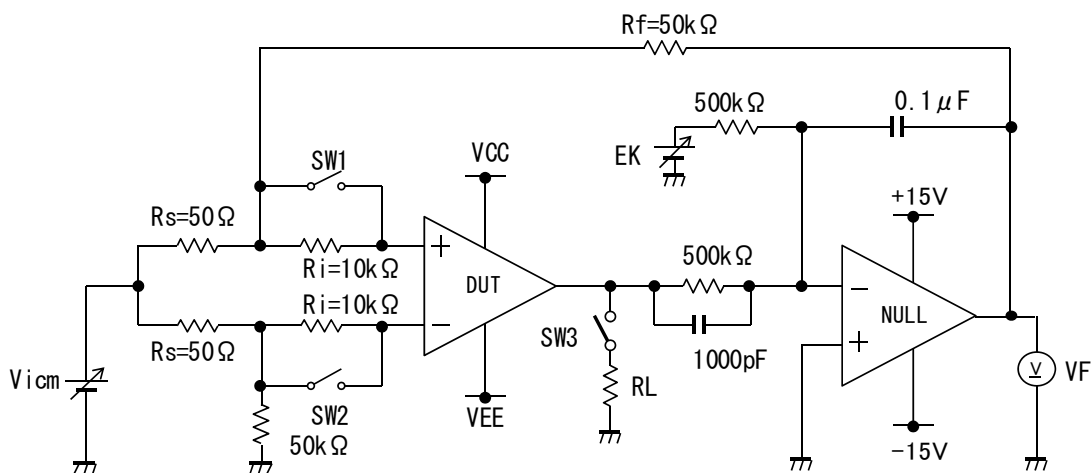
Figure 111. Test Circuit1 (One Channel Only)
