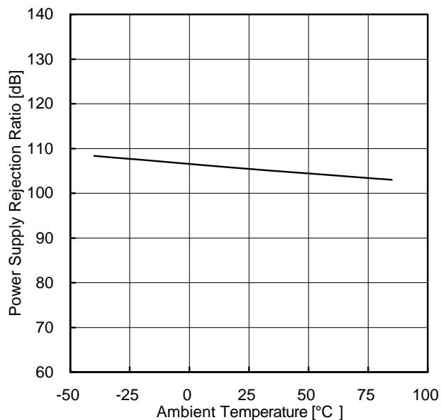
Figure 62. Power Supply Rejection Ratio vs Ambient Temperature
