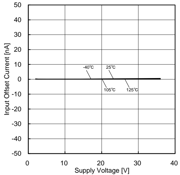
Figure 76. Input Offset Current vs Supply Voltage
