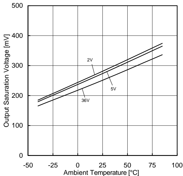
Figure 29. Output Saturation Voltage vs Ambient Temperature (I OL =4mA)
