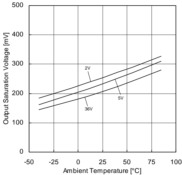
Figure 49. Output Saturation Voltage vs Ambient Temperature ( I_{OL}=4mA )
