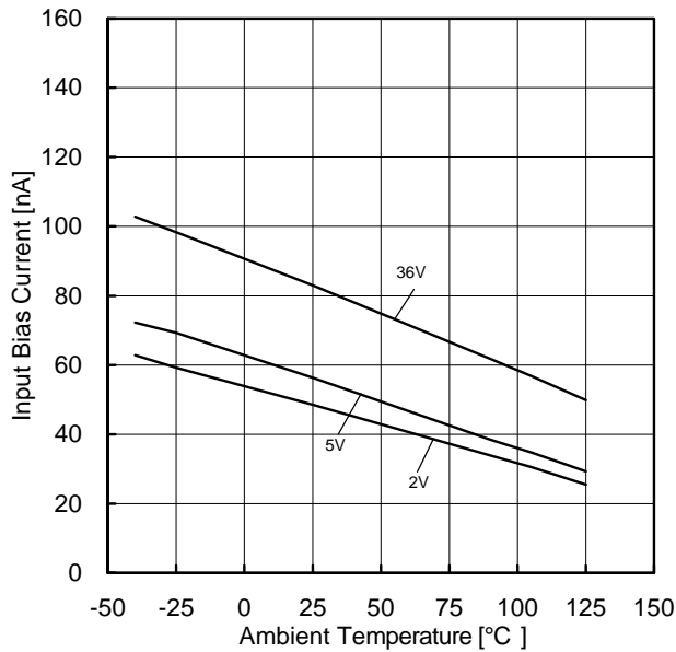
Figure 75. Input Bias Current vs Ambient Temperature
