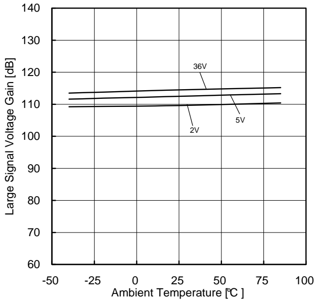
Figure 16. Large Signal Voltage Gain vs Ambient Temperature
