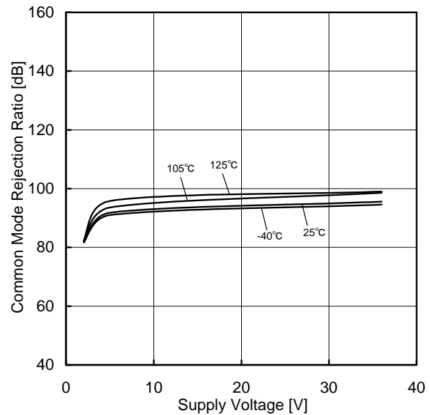
Figure 103. Common Mode Rejection Ratio vs Supply Voltage
