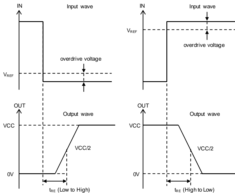
Figure 113. Response Time
