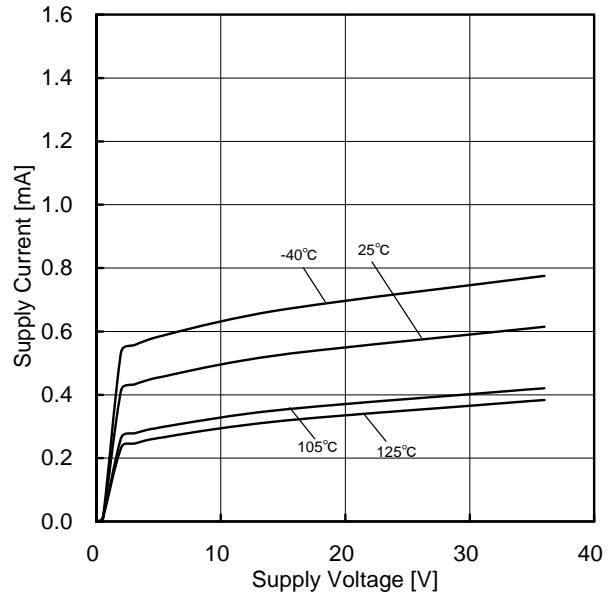
Figure 66. Supply Current vs Supply Voltage
