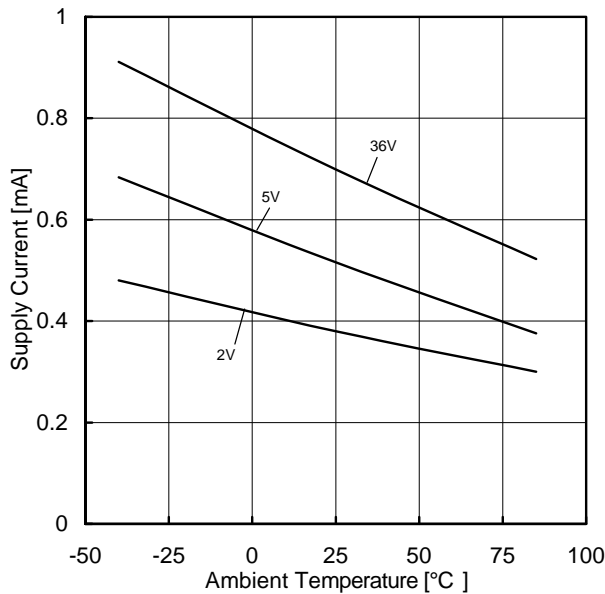
Figure 47. Supply Current vs Ambient Temperature
