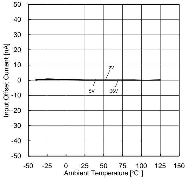
Figure 100. Input Offset Current vs Ambient Temperature
