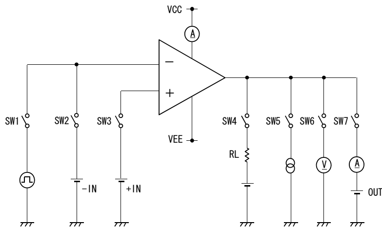
Figure 112. Test Circuit 2 (One Channel Only)
