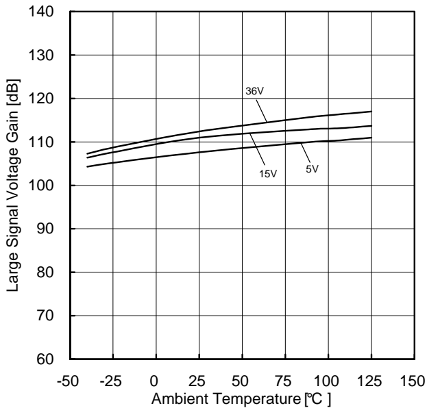
Figure 102. Large Signal Voltage Gain vs Ambient Temperature
