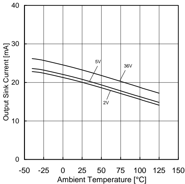
Figure 71. Output Sink Current vs Ambient Temperature (OUT=1.5V)
