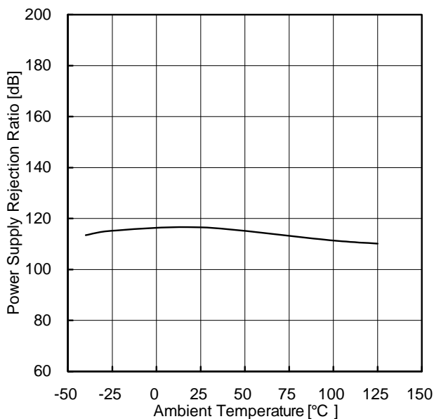
Figure 106. Power Supply Rejection Ratio vs Ambient Temperature
