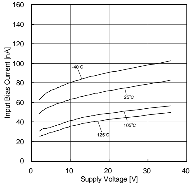
Figure 97. Input Bias Current vs Supply Voltage
