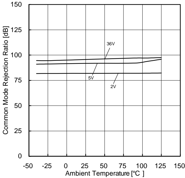
Figure 81. Common Mode Rejection Ratio vs Ambient Temperature
