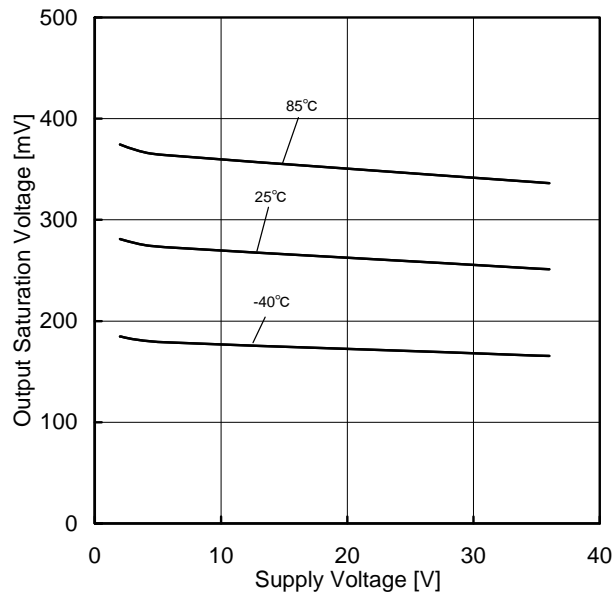
Figure 28. Output Saturation Voltage vs Supply Voltage ( I_{OL}=4mA )
