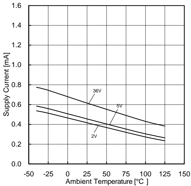
Figure 67. Supply Current vs Ambient Temperature
