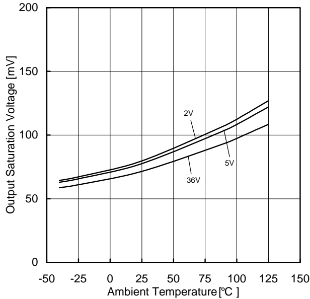
Figure 69. Output Saturation Voltage vs Ambient Temperature (I OL =4mA)
