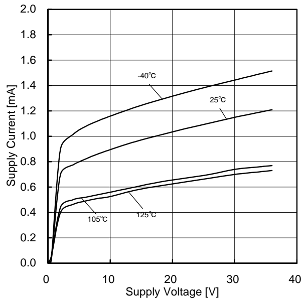
Figure 89. Supply Current vs Supply Voltage
