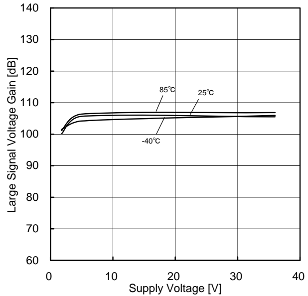
Figure 58. Large Signal Voltage Gain vs Supply Voltage
