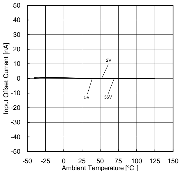
Figure 77. Input Offset Current vs Ambient Temperature
