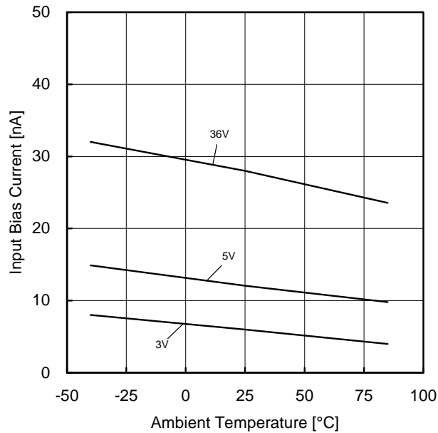
Figure 55. Input Bias Current vs Ambient Temperature
