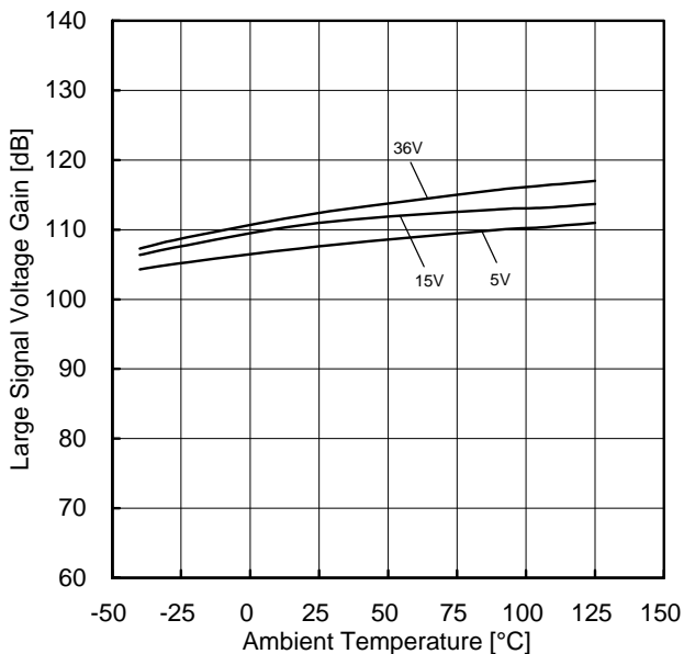
Figure 79. Large Signal Voltage Gain vs Ambient Temperature
