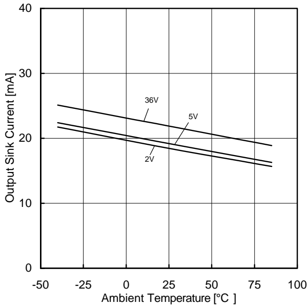
Figure 8. Output Sink Current vs Ambient Temperature ( OUT=1.5V )
