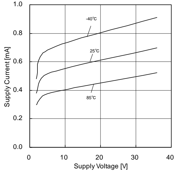
Figure 46. Supply Current vs Supply Voltage
