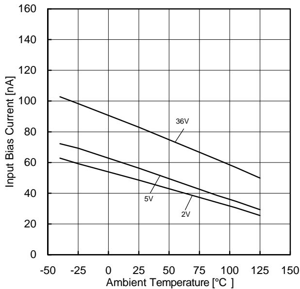
Figure 98. Input Bias Current vs Ambient Temperature
