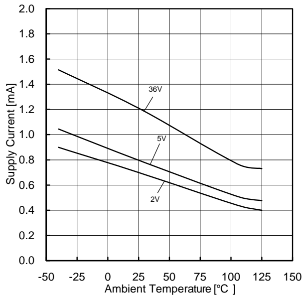
Figure 90. Supply Current vs Ambient Temperature
