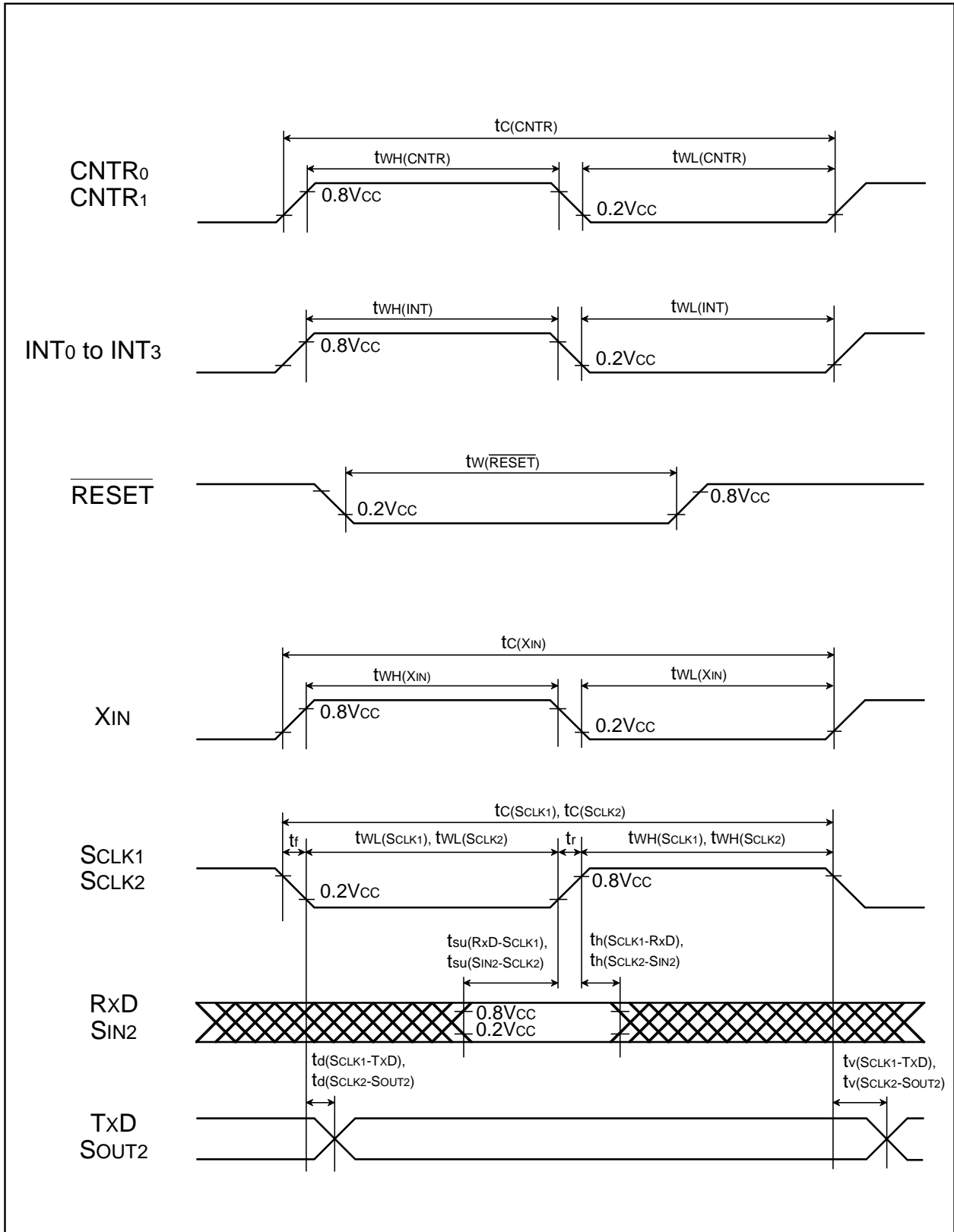
Fig. 81 Timing diagram
