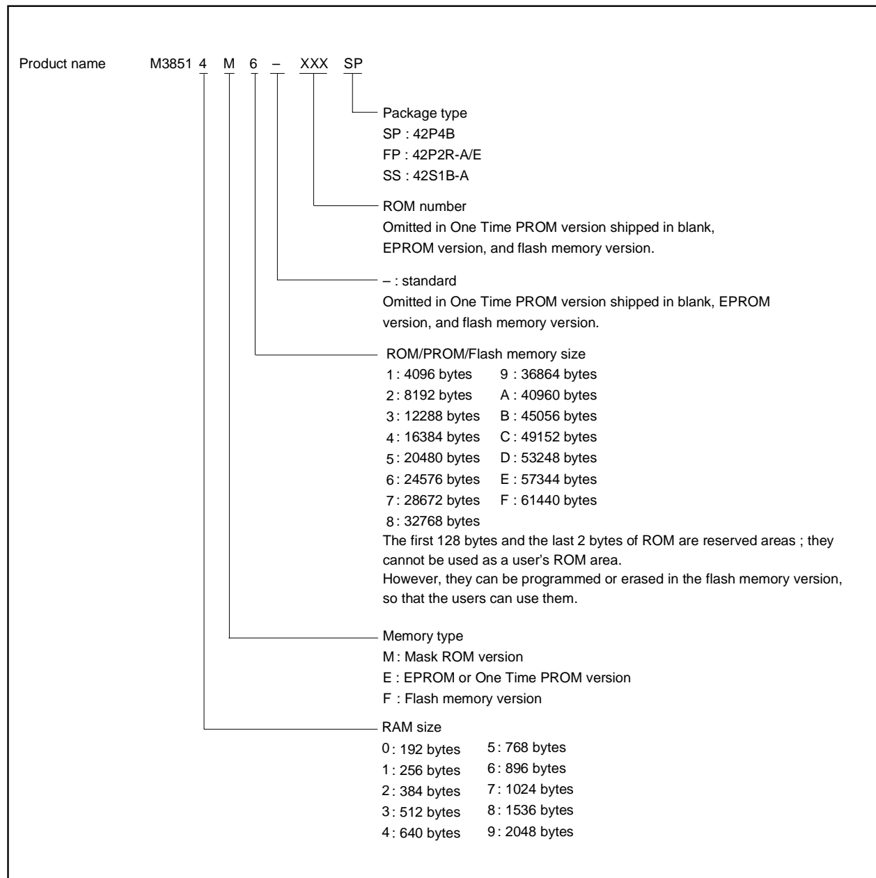
Fig. 3 Part numbering
