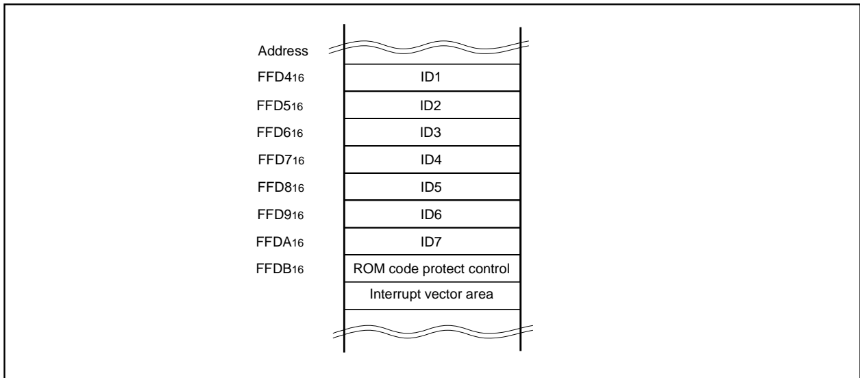
Fig. 74 ID code storage addresses
