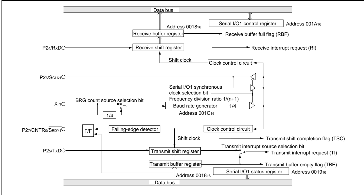
Fig. 18 Block diagram of clock synchronous serial I/O1
