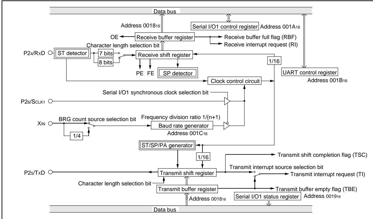
Fig. 20 Block diagram of UART serial I/O1
