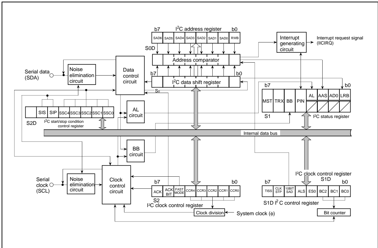
Fig. 27 Block diagram of multi-master I 2 C-BUS interface
