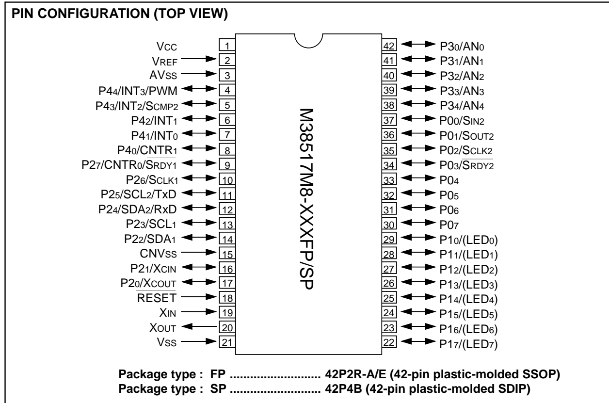
Fig. 1 M38517M8-XXXXFP/SP pin configuration
