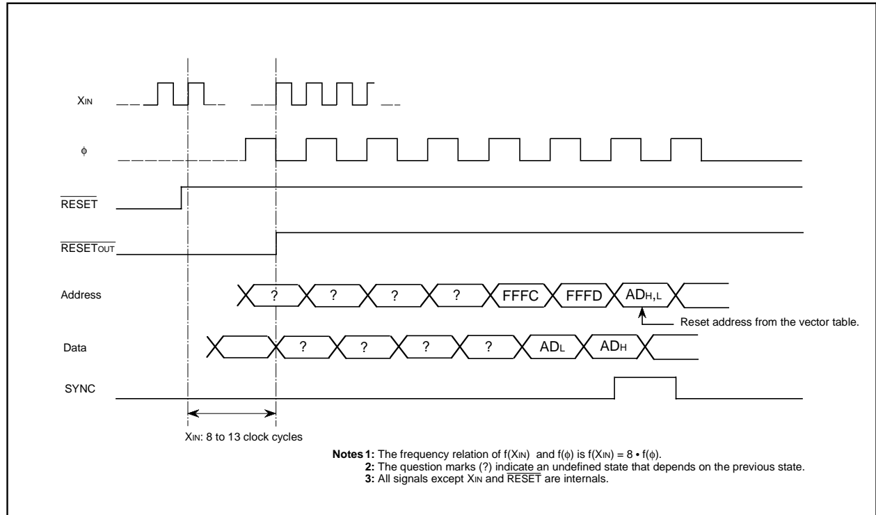
Fig. 50 Reset sequence
