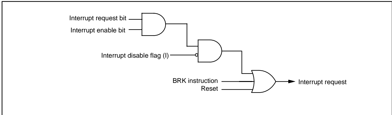
Fig. 13 Interrupt control
