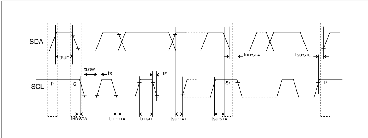
Fig. 78 Timing diagram of multi-master I 2 C-BUS
