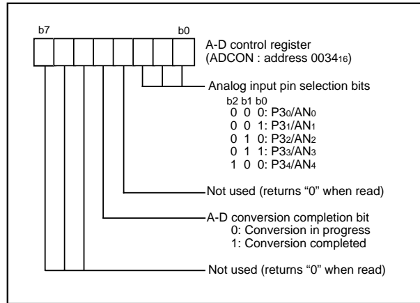
Fig. 44 Structure of A-D control register
