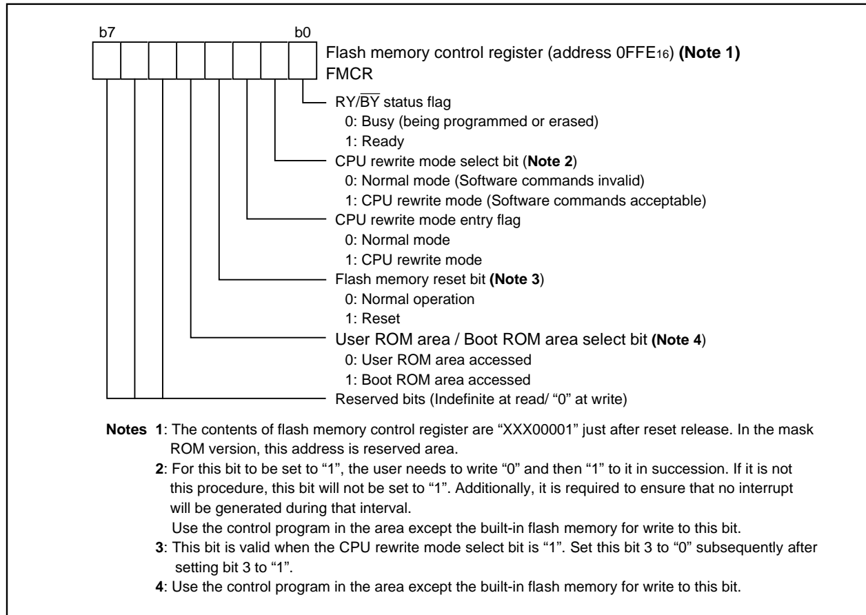
Fig. 58 Structure of flash memory control register
