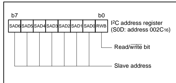
Fig. 28 Structure of I 2 C address register
