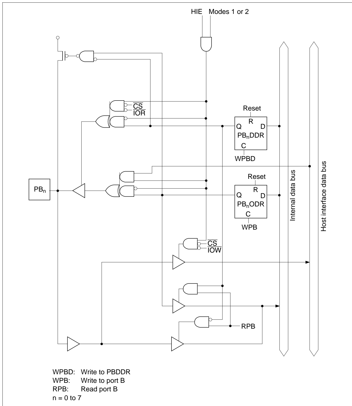
Figure C.11 Port B Block Diagram
