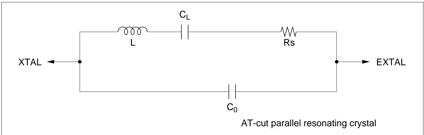
Figure 6.3 Equivalent Circuit of External Crystal
