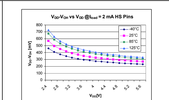
Figure 18. Typical V_{DD}-V_{OH} vs. V_{DD} at I_{load} = 2 mA
