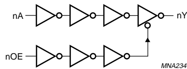
Fig.5 Logic diagram.
