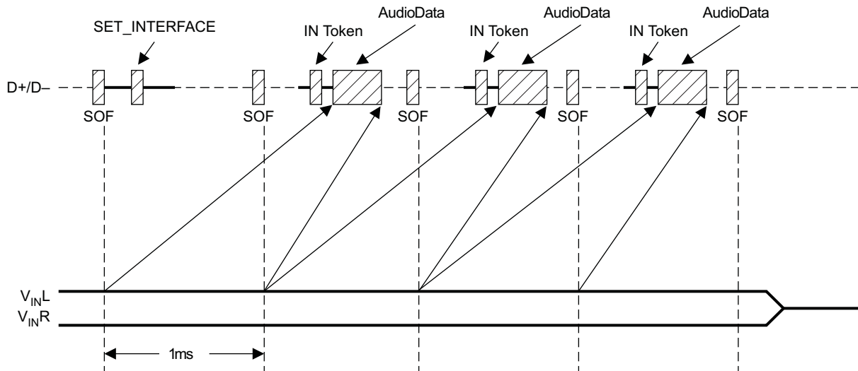
Figure 38. Record Sequence
