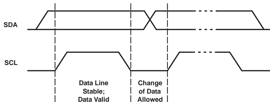
Figure 2. Bit Transfer
