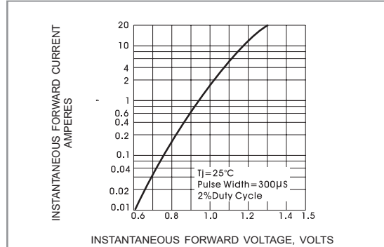
Fig.2- TYPICAL INSTANTANEOUS FORWARD CHARACTERISTIC
