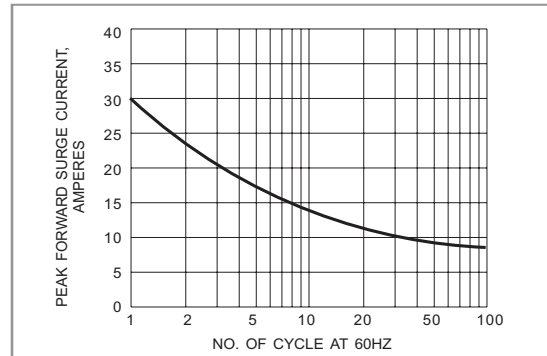
Fig.4- MAXIMUM NON - REPETITIVE SURGE CURRENT
