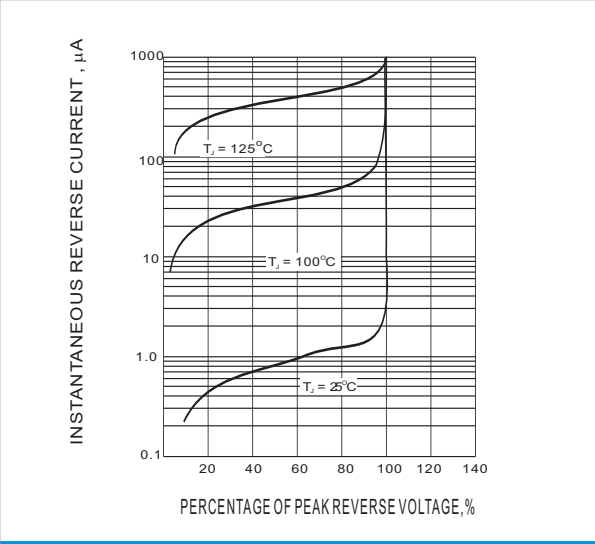
Fig.3-TYPICAL REVERSE CHARACTERISTIC
