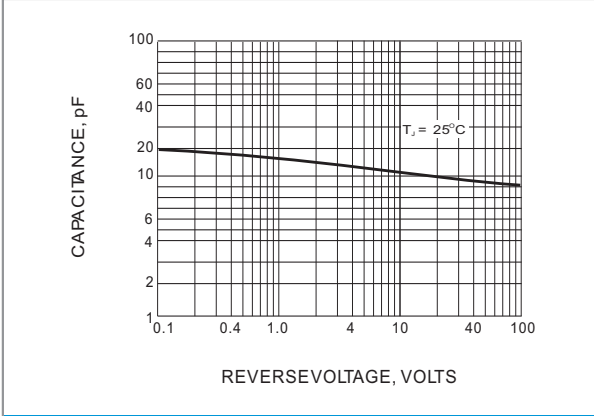
Fig.5-TYPICAL JUNCTION CAPACITANCE
