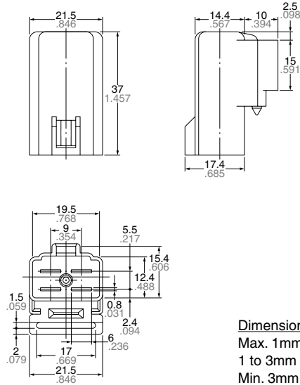
External dimensions
