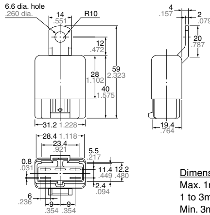
External dimensions
