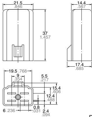
External dimensions
