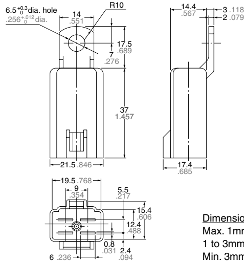
External dimensions
