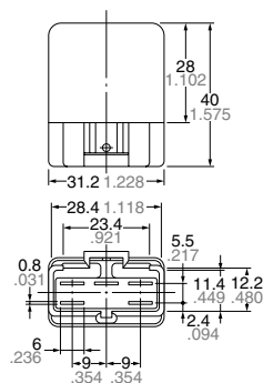
External dimensions
