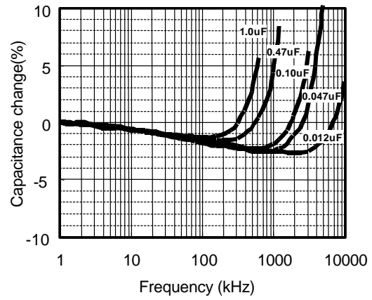
Frequency Characteristics
