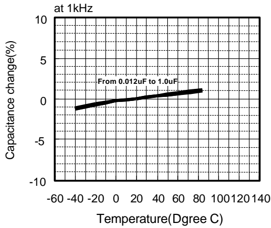
Temperature Characteristics
