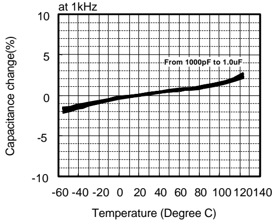
Temperature Characteristics
