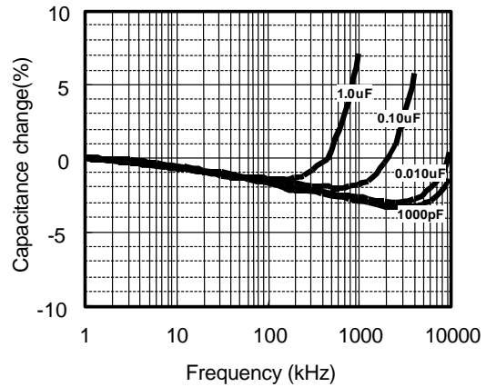
Frequency Characteristics
