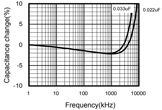
Frequency Characteristics
