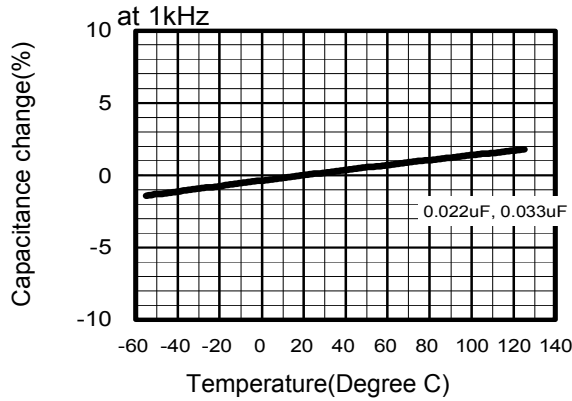
Temperature Characteristics
