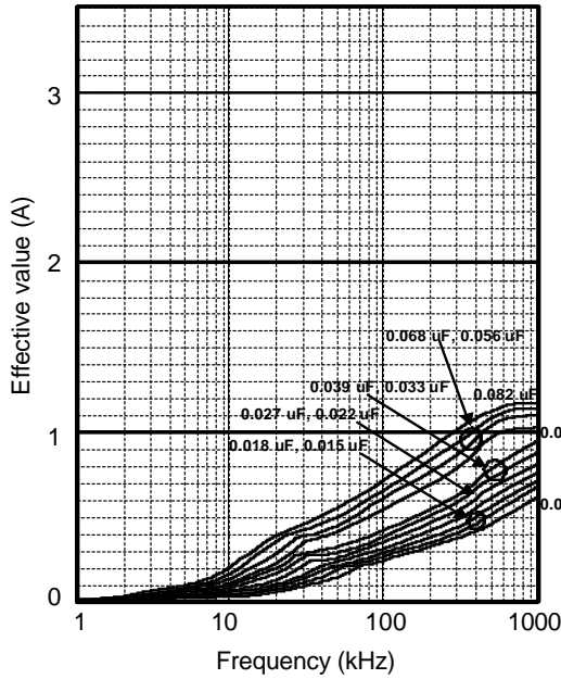
Permissible current
