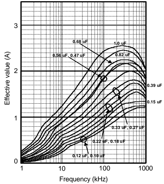
Permissible current
