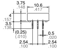
Self-clinching terminal
