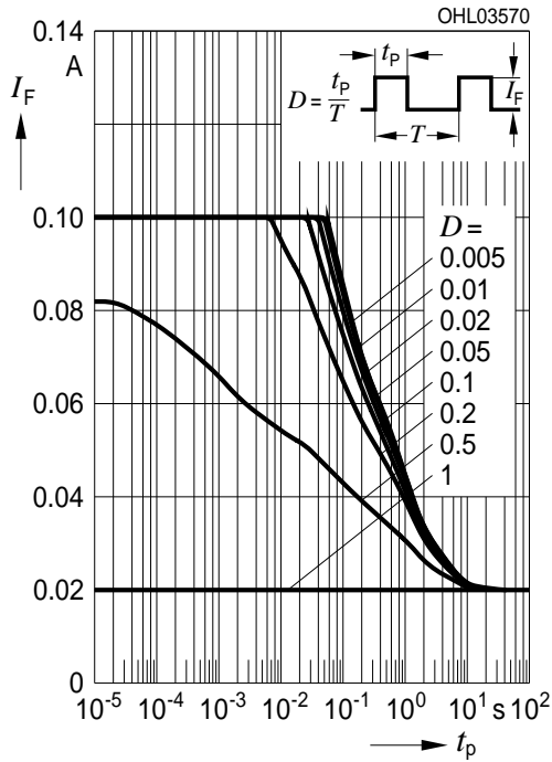
Zulässige Impulsbelastbarkeit Permissible Pulse Handling Capability Duty cycle D = parameter, T_A = 85\text{ °C} I_F = f(t_p) ; blue (1 Chip on)
