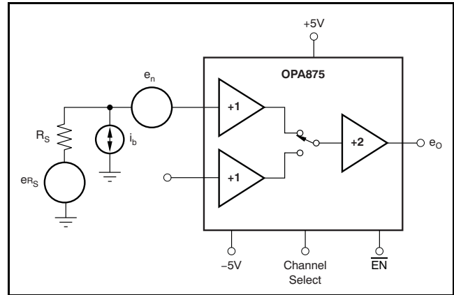
Figure 30. Noise Model
