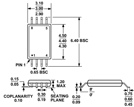
Figure 3. 8-Lead Thin Shrink Small Outline Package [TSSOP] (RU-8)
