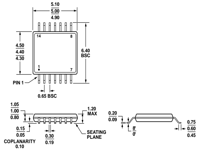
Figure 4. 14-Lead Thin Shrink Small Outline Package [TSSOP] (RU-14)
