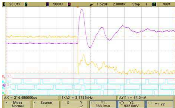
Figure 12. Typical Transient Response for Design Example Load Step
