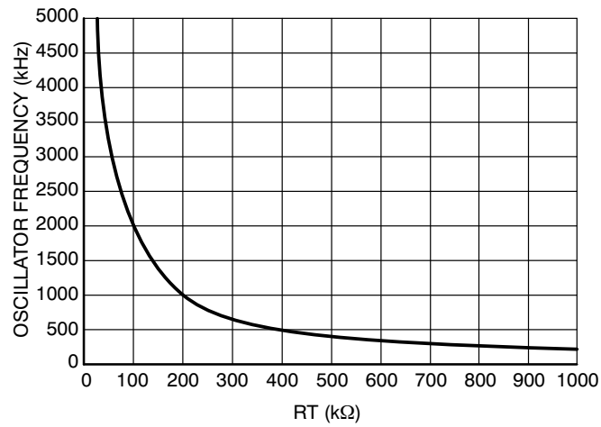
Figure 3. Oscillator Frequency vs. RT
