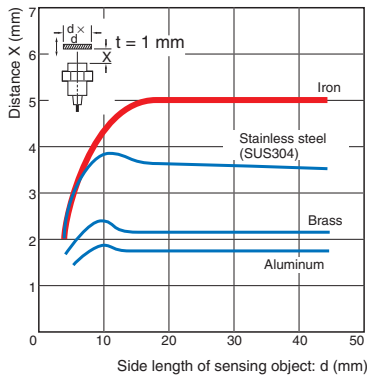
E2E-X5ME/-X5MY/-X5MF
