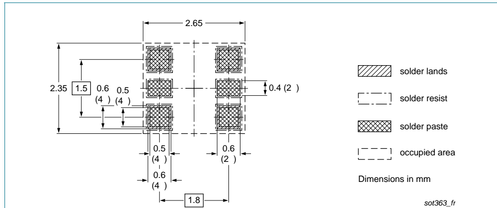
Fig 19. Reflow soldering footprint PUMD13 (SOT363)
