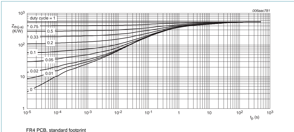
Fig 2. Transient thermal impedance from junction to ambient as a function of pulse duration for PDTC144EE (SOT416); typical values
