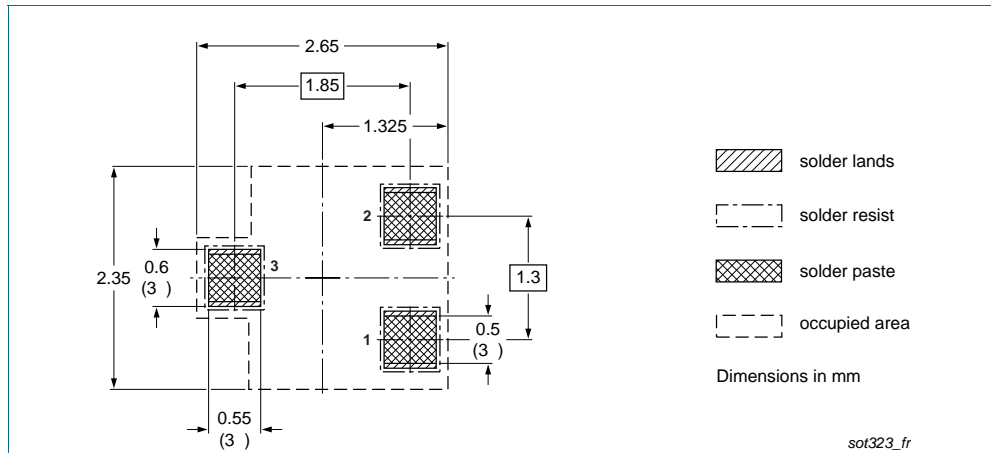
Fig 20. Reflow soldering footprint PDTC144EU (SOT323/SC-70)
