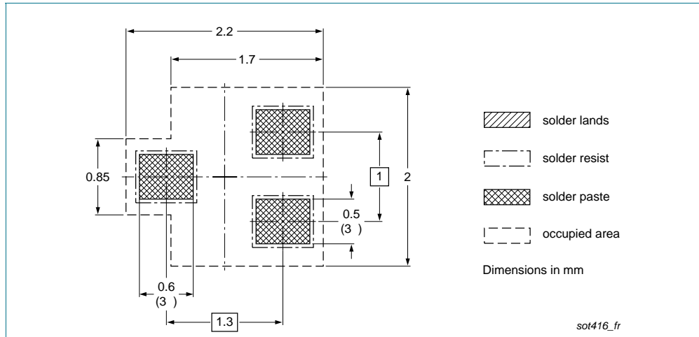
Fig 16. Reflow soldering footprint PDTC144EE (SOT416/SC-75)
