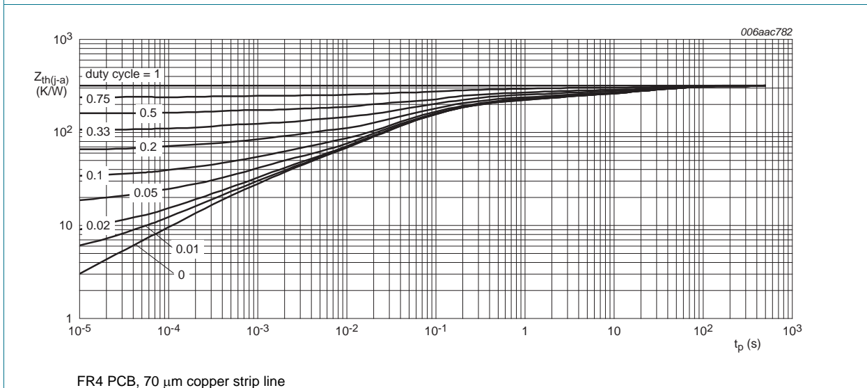
Fig 3. Transient thermal impedance from junction to ambient as a function of pulse duration for PDTC124EM (SOT883); typical values
