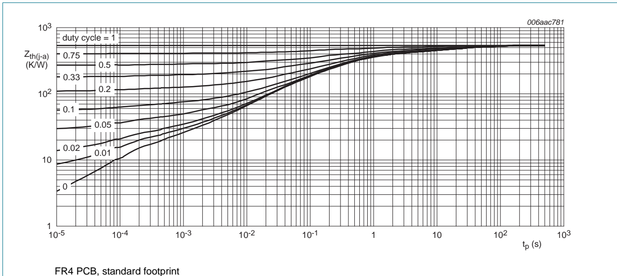
Fig 2. Transient thermal impedance from junction to ambient as a function of pulse duration for PDTC124EE (SOT416); typical values
