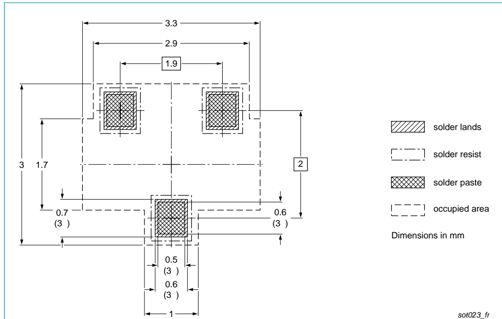
Fig 18. Reflow soldering footprint PDTC124ET (SOT23)
