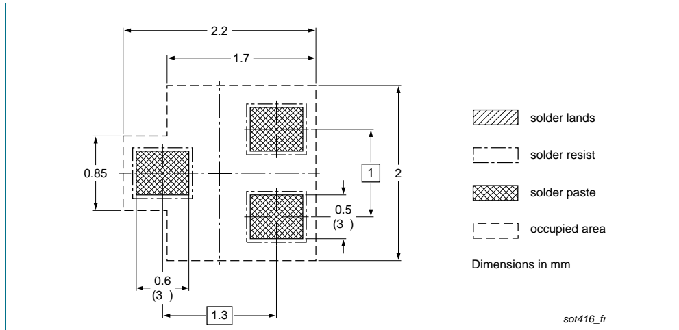
Fig 16. Reflow soldering footprint PDTC124EE (SOT416/SC-75)
