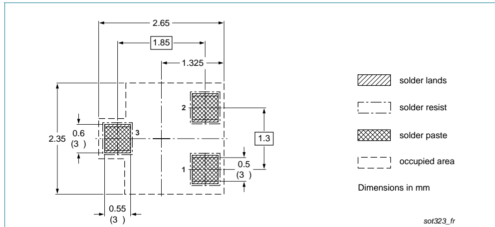
Fig 20. Reflow soldering footprint PDTC124EU (SOT323/SC-70)
