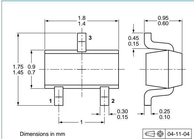
Fig 3. Package outline SOT416 (SC-75)
