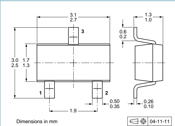
Fig 4. Package outline SOT346 (SC-59A/TO-236)
