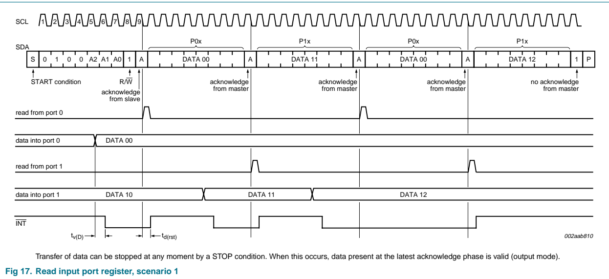
Fig 17. Read input port register, scenario 1
