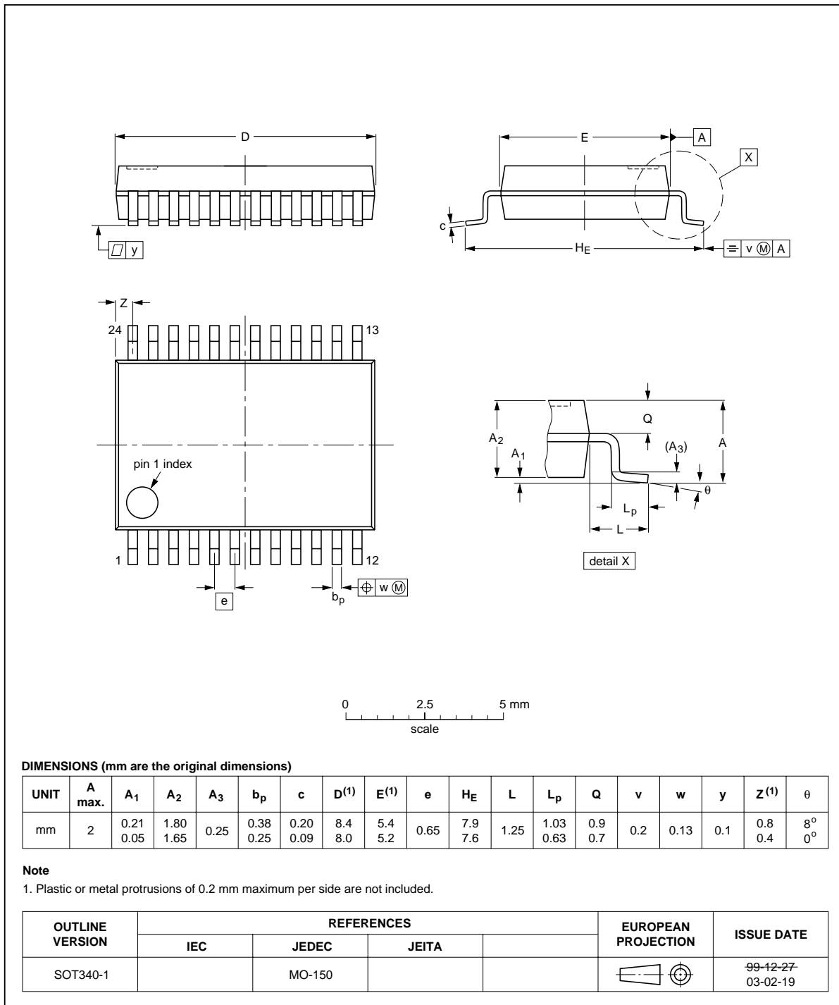
Fig 28. Package outline SOT340-1 (SSOP24)
