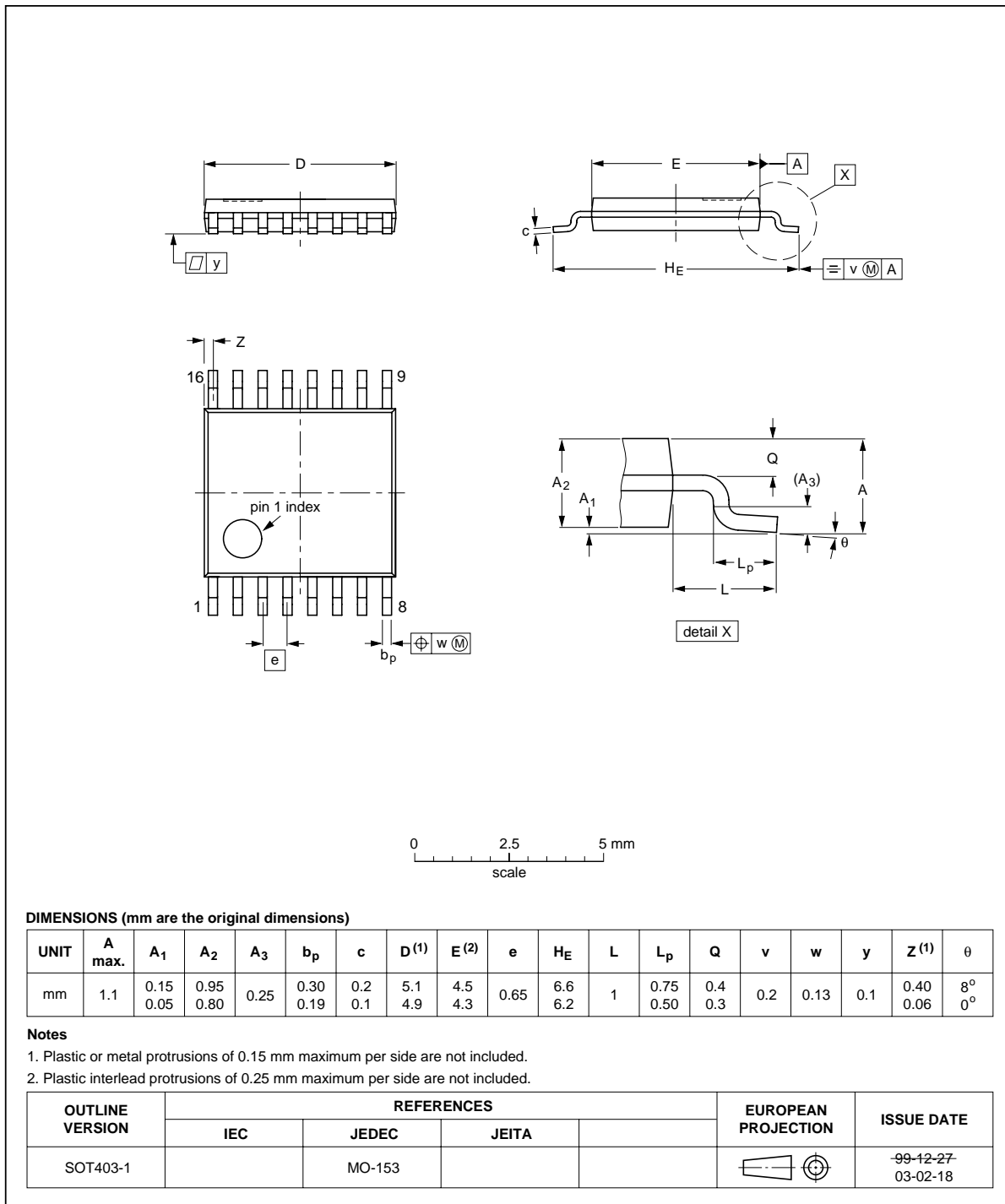
Fig 24. Package outline SOT403-1 (TSSOP16)
