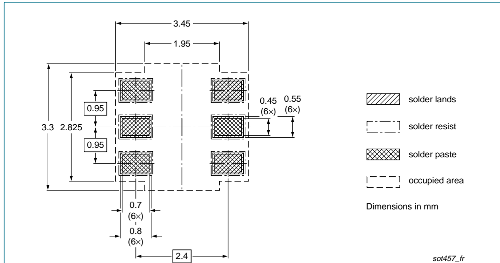
Fig 18. Reflow soldering footprint SOT457 (SC-74)
