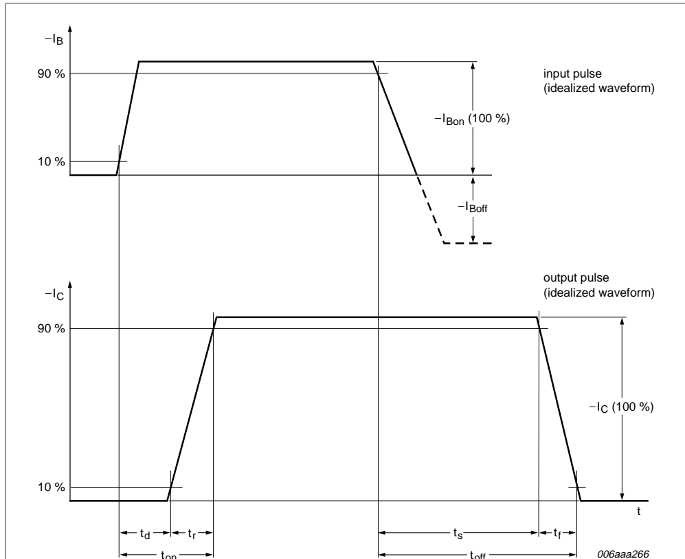
Fig 17. BISS transistor switching time definition
