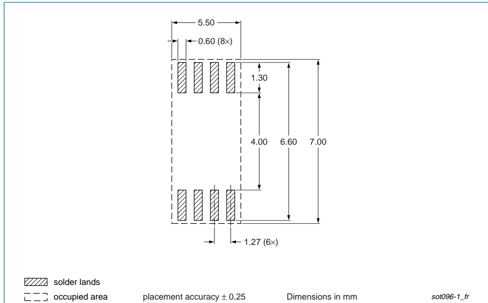
Fig 20. Reflow soldering footprint SOT96-1 (SO8)
