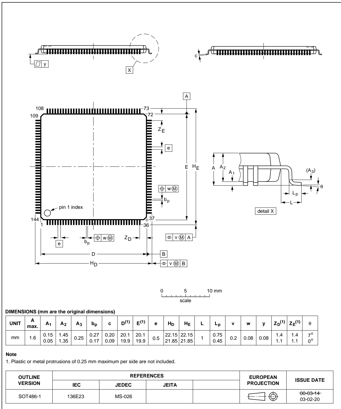
Fig 51. Package outline for the LQFP144 package
