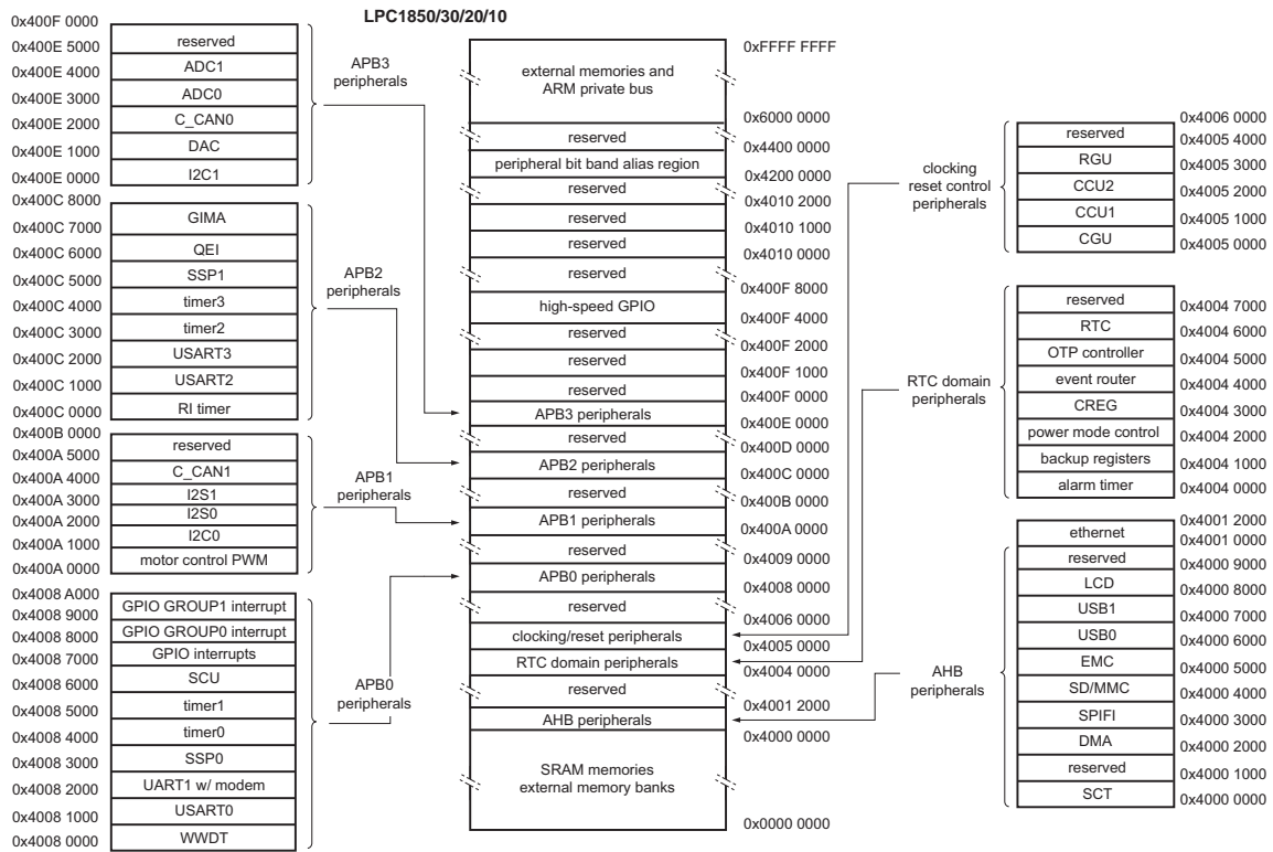
Fig 9. LPC1850/30/20/10 Memory mapping (peripherals)
