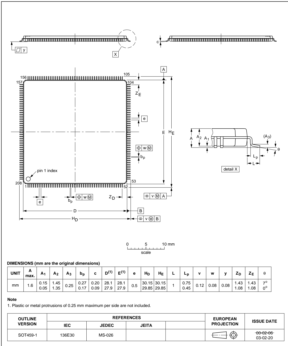
Fig 49. Package outline of the LQFP208 package
