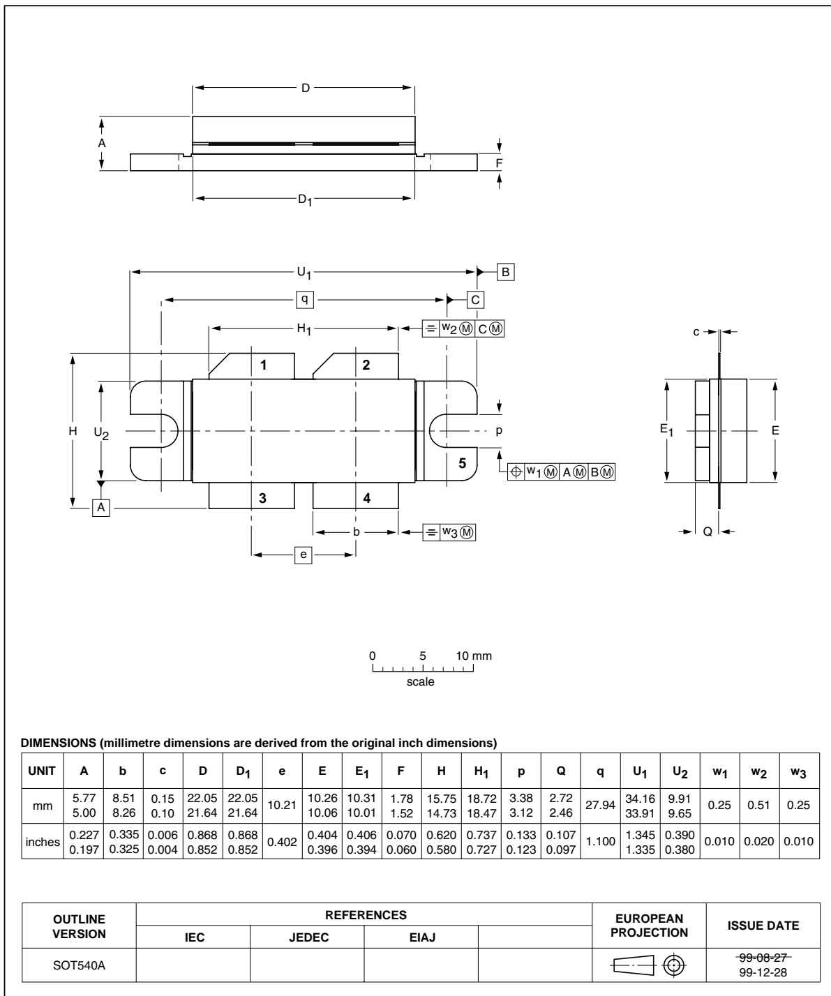
Fig 9. Package outline SOT540A
