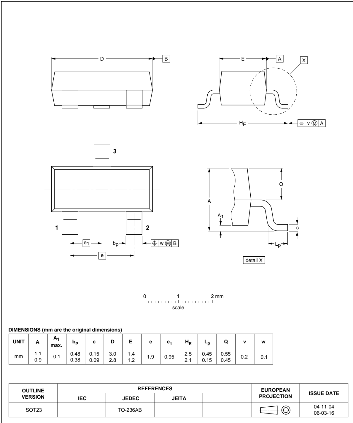
Fig 23. Package outline.
