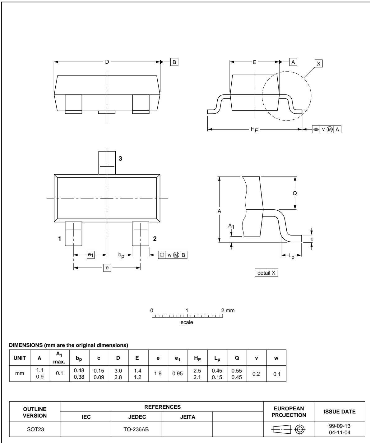
Fig 13. Package outline SOT23 (TO-236AB).
