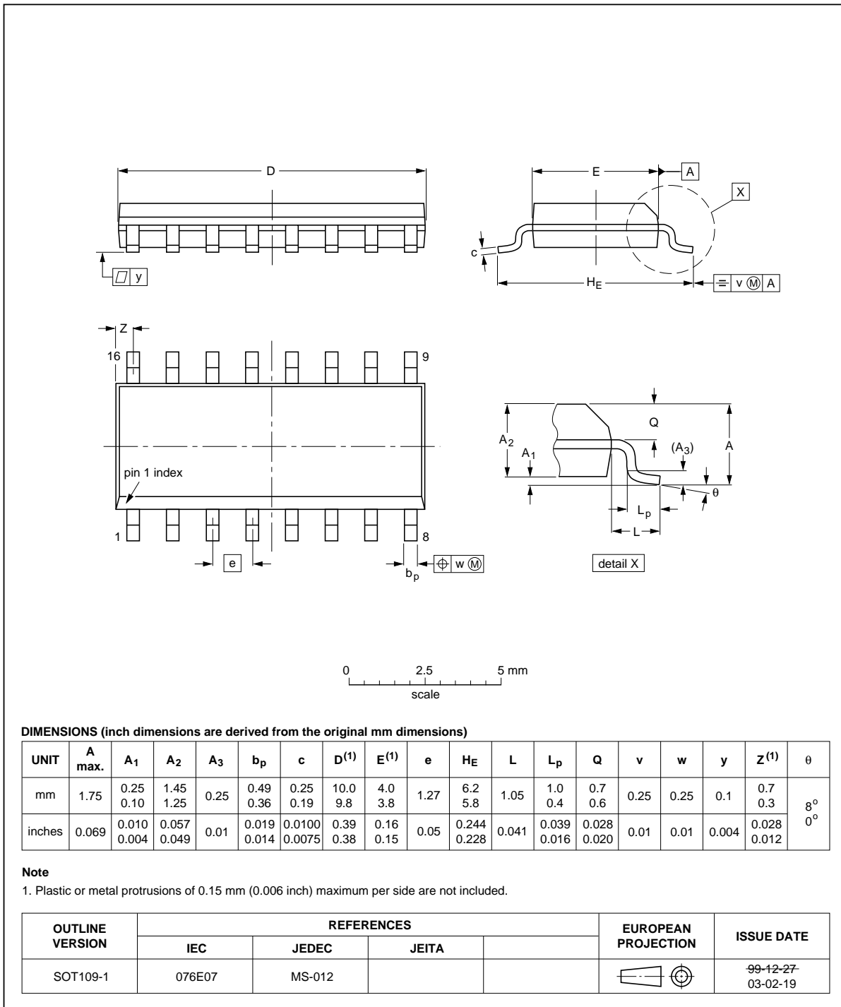
Fig 21. Package outline SOT109-1 (SO16)
