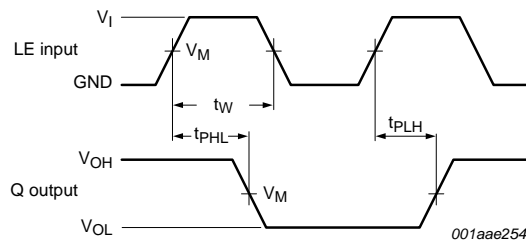
Fig 8. The latch enable input (LE) to output (Q) propagation delays, the latch enable input (LE) pulse width
