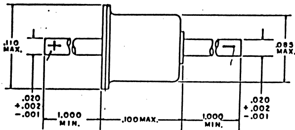
AXIAL DIODE OUTLINE
