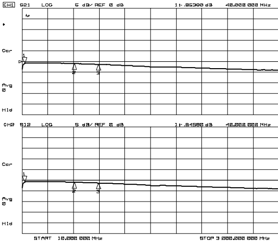
S21, S12 (f=10MHz~3GHz)
