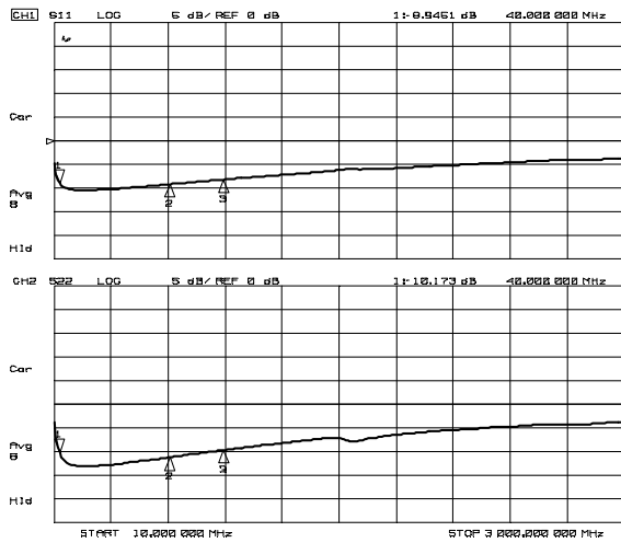
S11, S22 (f=10MHz~3GHz)
