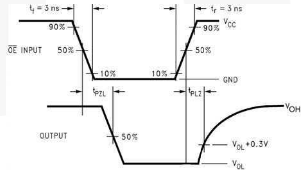
Figure 6. AC Waveforms
