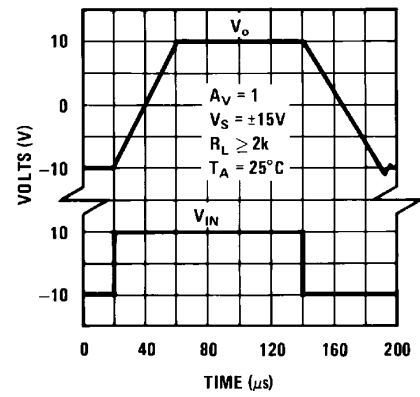
Large Signal Pulse Response (LM148)
