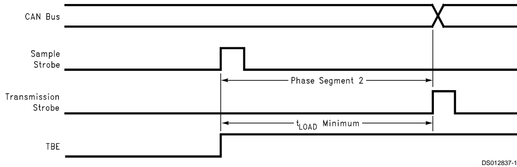
FIGURE 16. TBE Timing
