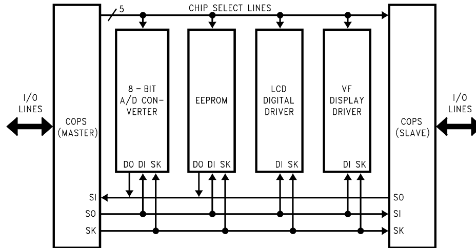
FIGURE 35. MICROWIRE/PLUS Application
