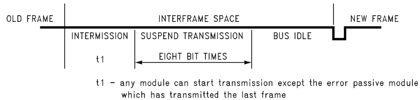
FIGURE 23. Interframe Space for Nodes Which Are Error Passive and Have Been Transmitter for the Last Frame
