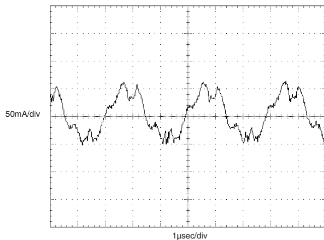
(VIN = 24V, 5V @ 15A, 3.3V @ 0A, external 22μF low-ESR input capacitor.)
