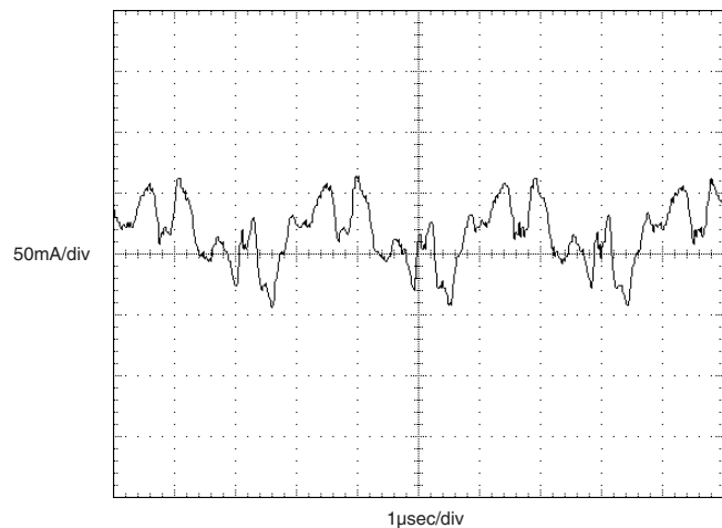
(VIN = 48V, 5V @ 15A, 3.3V @ 0A, external 22μF low-ESR input capacitor.)
