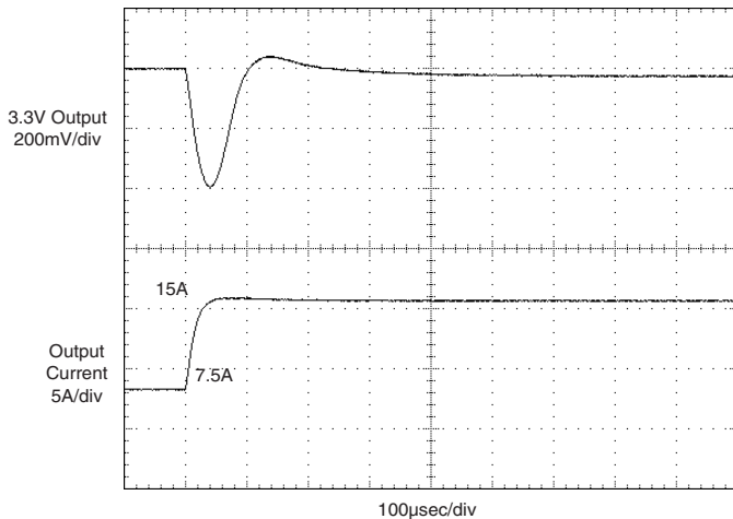
3.3V Output Half-Load to Full-Load Transient Response (VIN = 24V, 5V @ 0A, external 10μF || 1μF output capacitors.)
