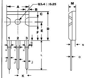
TO-247 (3P)
