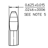
DETAIL "Y" SCALE 30:1
