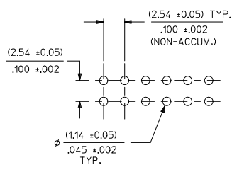
PCB LAYOUT: COMPONENT SIDE TYPICAL PCB THICKNESS: (1.57)/.062
