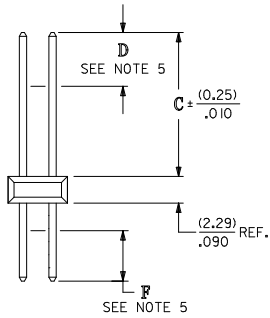
DETAIL "Y" SCALE 30:1
