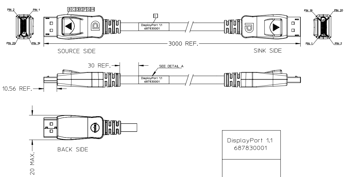
DETAIL A
