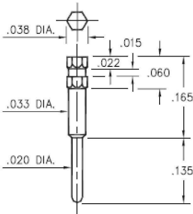
4366-0-00-XX-00-00-03-0 Hex press-fit in .034 plated thru hole
