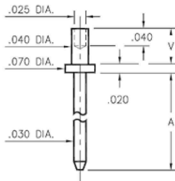
311X-X-00-XX-00-00-08-0 Swage mount in .043 hole
