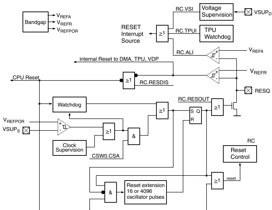
Fig. 5–3: Block diagram of reset logic
