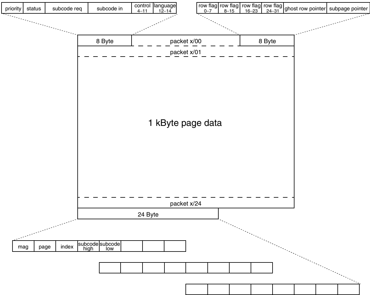
Fig. 3–5: Page format
