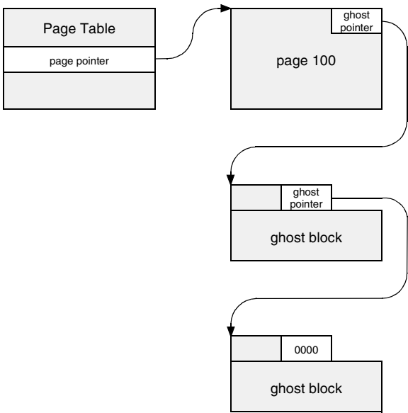
Fig. 3–6: Ghost row organization
