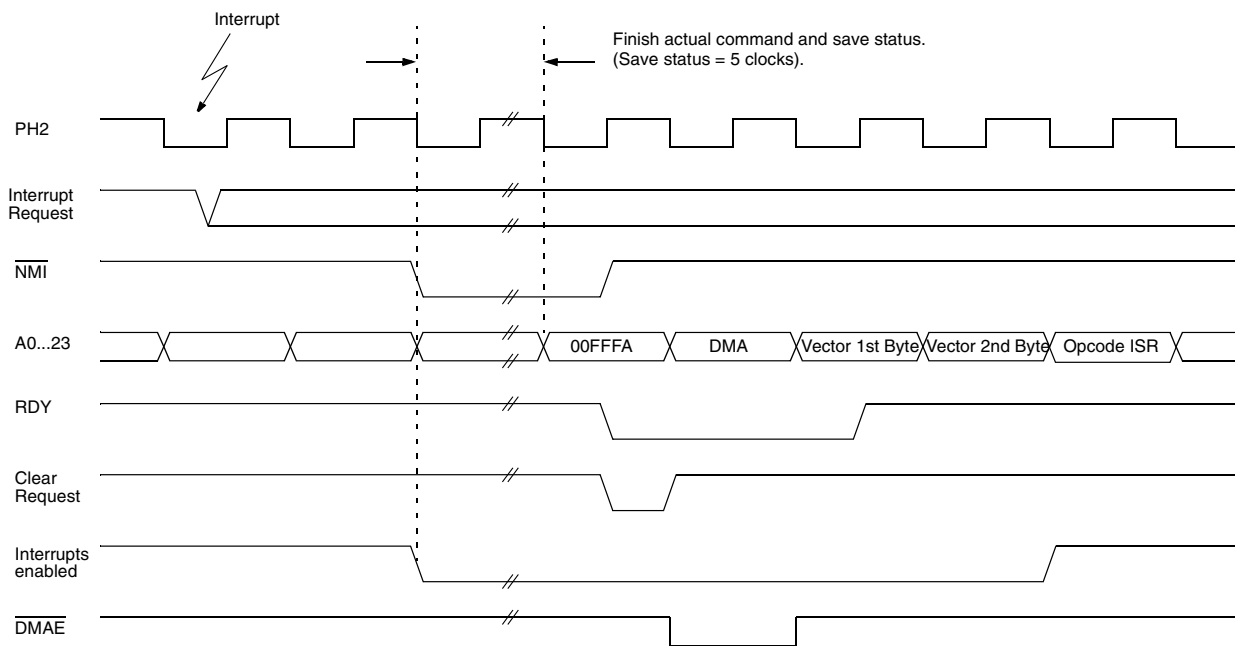
Fig. 5–15: Interrupt timing diagram
