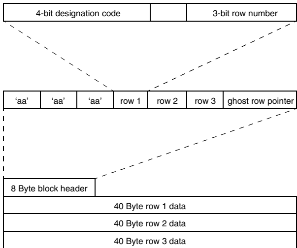
Fig. 3–7: Ghost block structure
