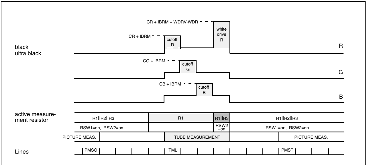
Fig. 2–20: MADC measurement timing
