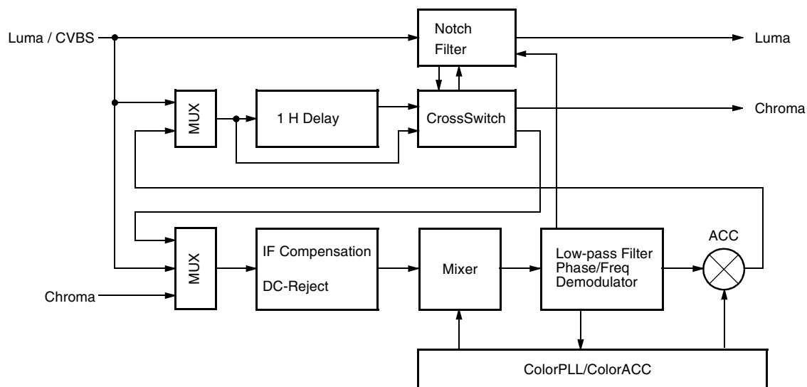
Fig. 2–4: Color decoder
