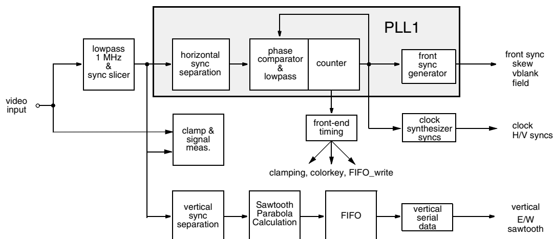
Fig. 2–10: Sync separation block diagram
