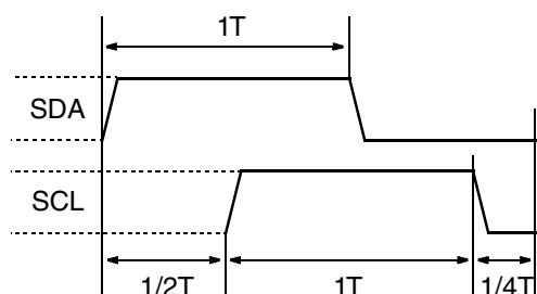
Fig. 5–19: Start condition I²C bus
