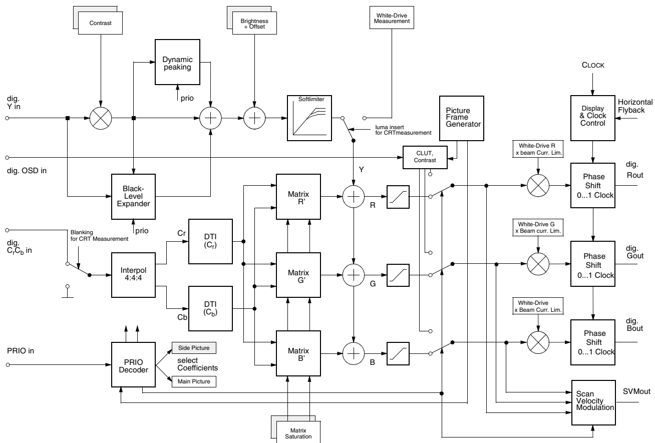
Fig. 2-18: Digital back-end
