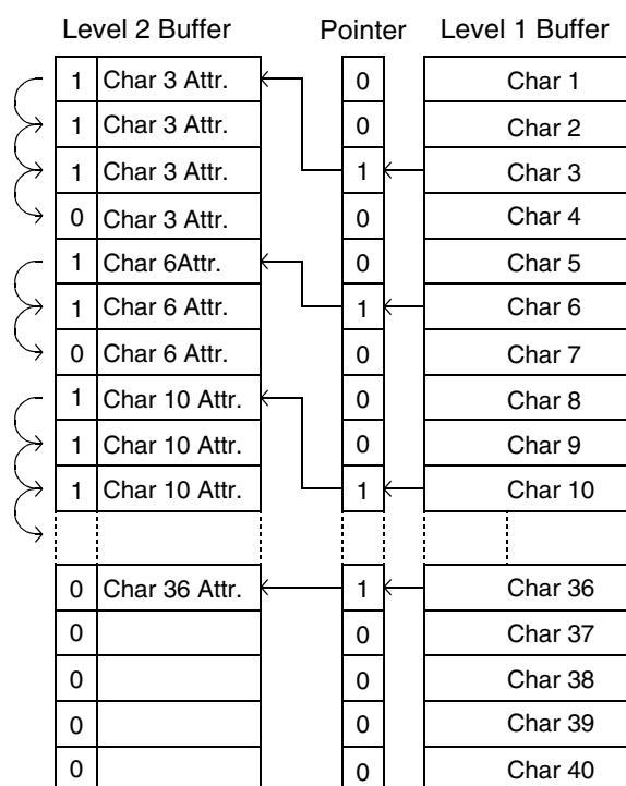
Fig. 3–9: Stack Row Buffer
