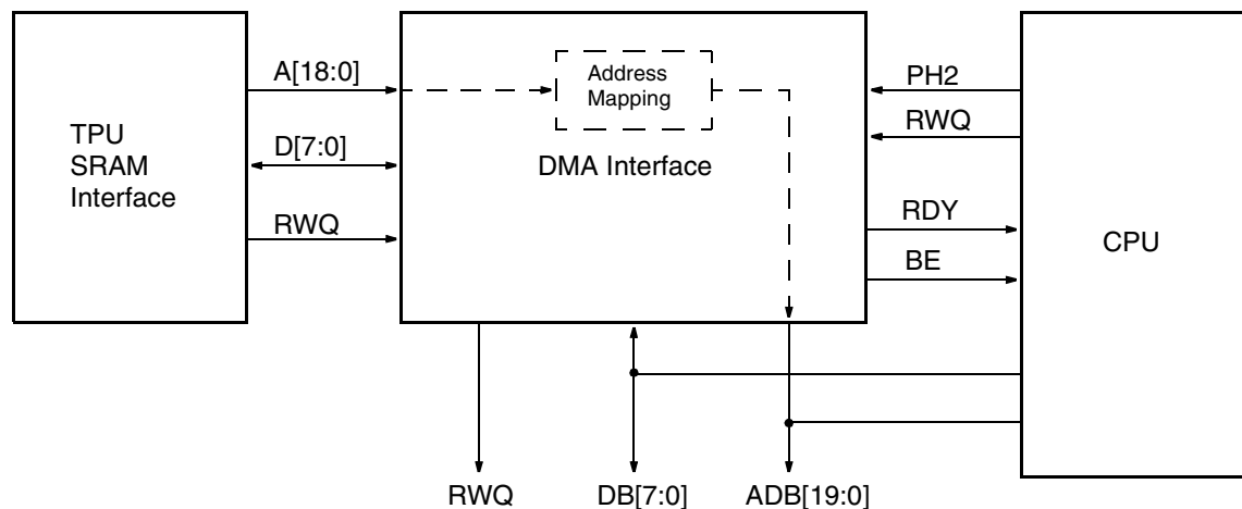
Fig. 5–7: Block diagram of DMA interface
