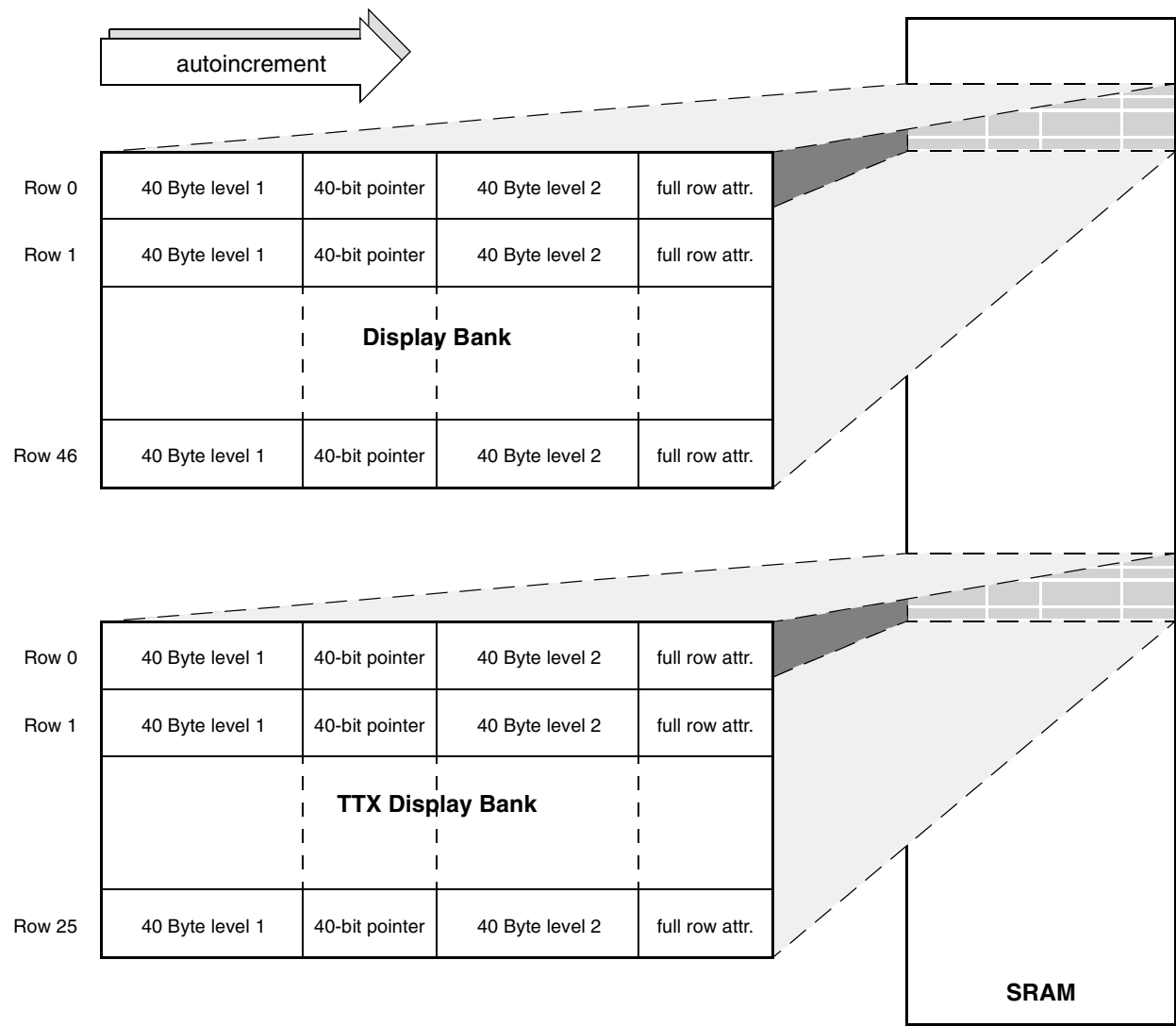
Fig. 3–10: Display memory organization (level 2)
