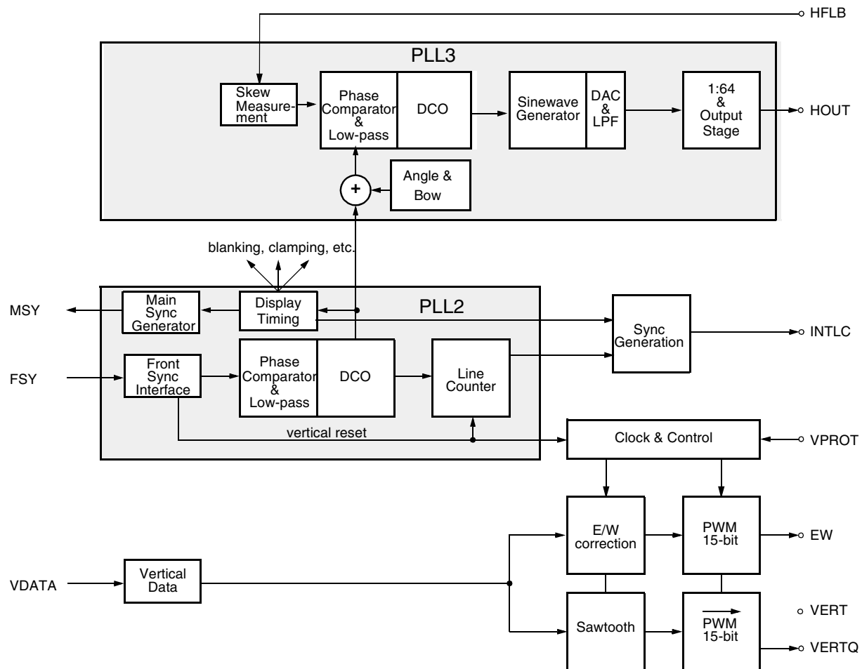
Fig. 2–24: Deflection processing block diagram
