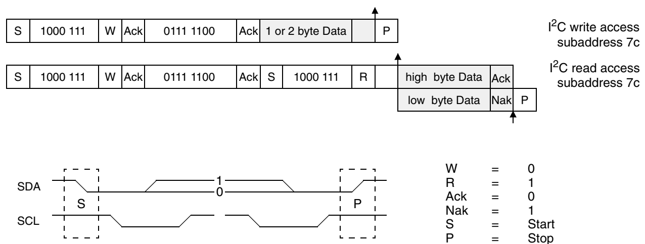
Fig. 2–26: I 2 C bus protocols
