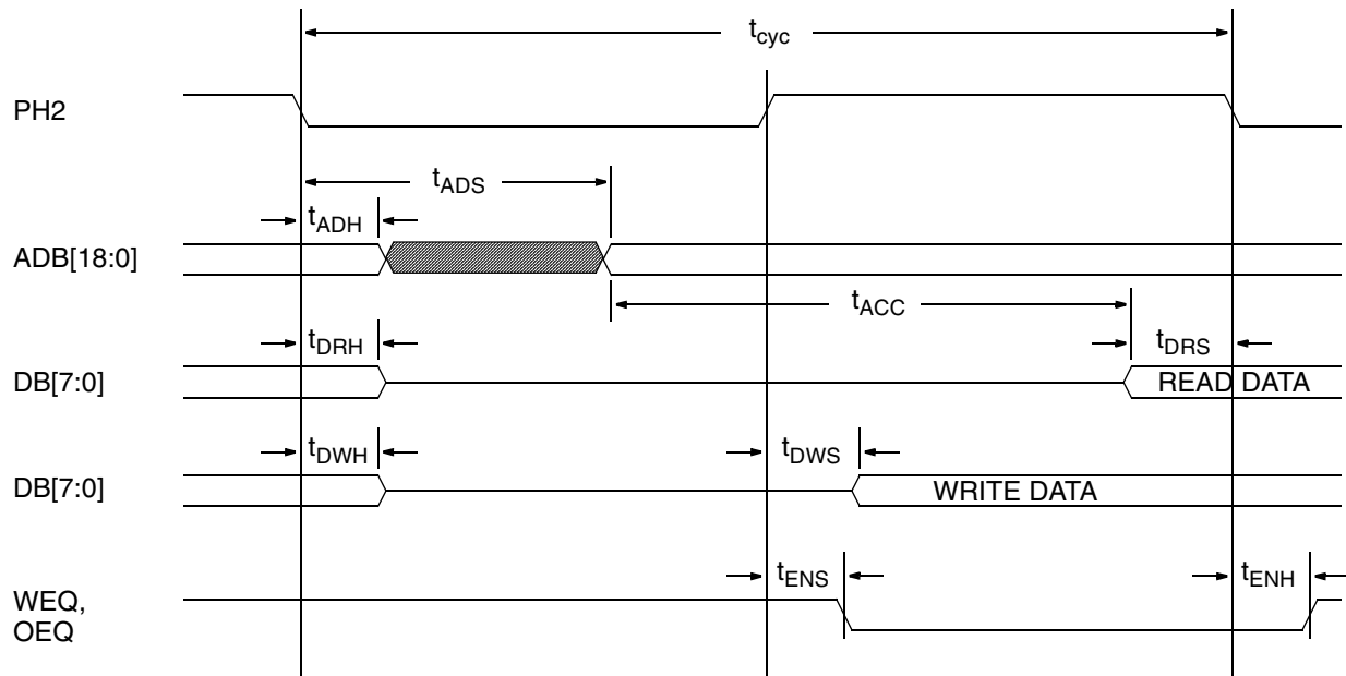
Fig. 6–32: Memory port timing
