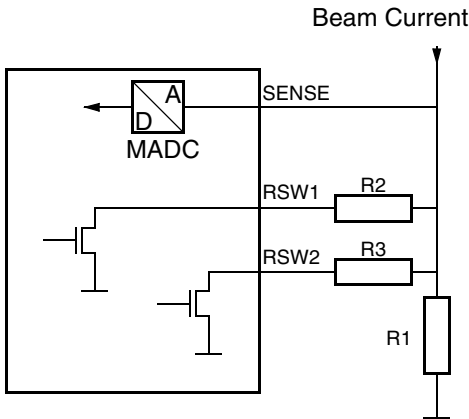
Fig. 2–19: MADC range switches
