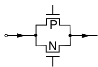
Fig. 6–23: Input pin SENSE
