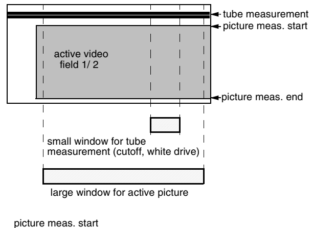
Fig. 2–21: Windows for tube and picture measurements
