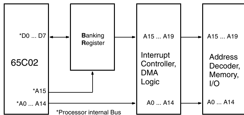
Fig. 5-5: Block diagram of Memory Banking
