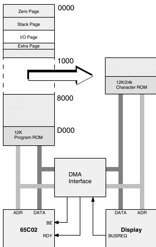
Fig. 3-2: Memory environment of text controller
