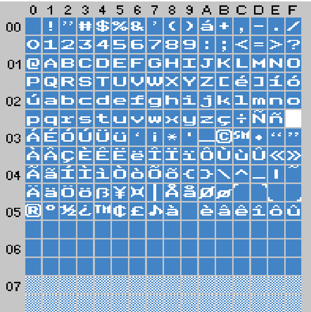
Fig. 3–16: Character font ROM for Closed Caption
