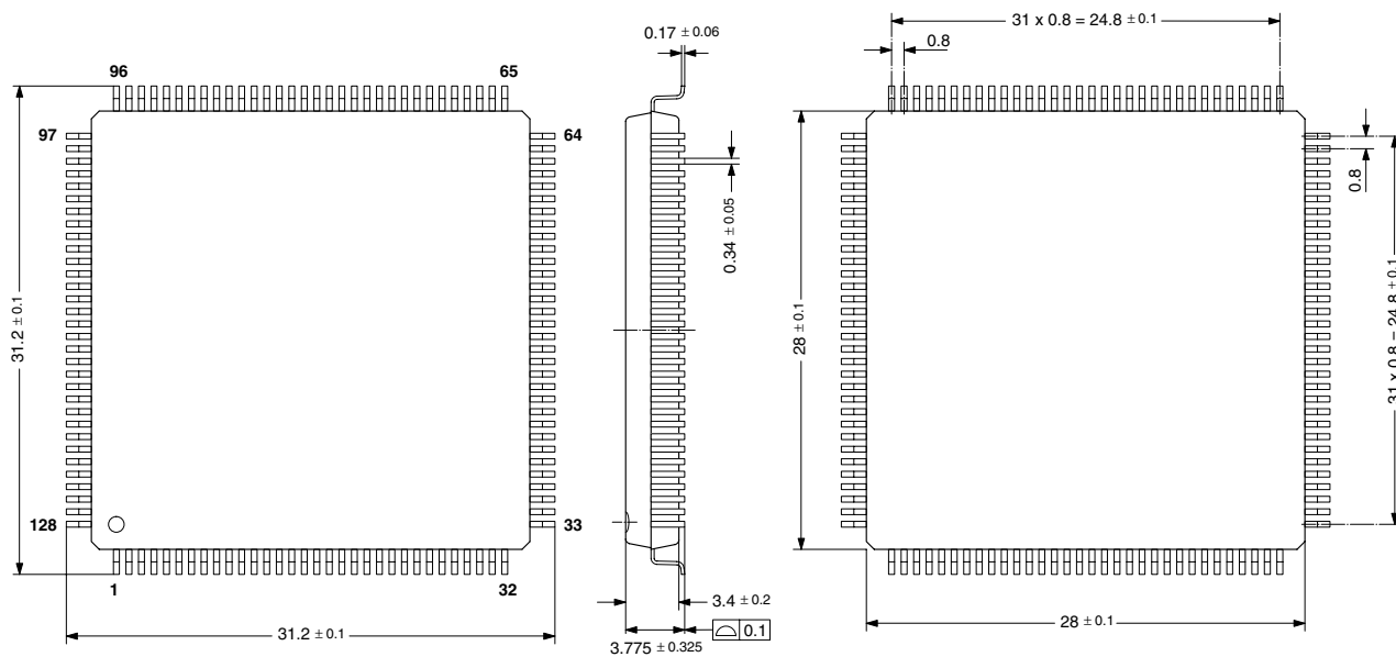
Fig. 6-2: 128-Pin Plastic Metric Quad Flat Package (PMQFP128)
