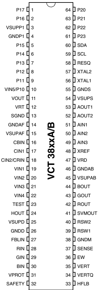
Fig. 6–3: PSDIP64 package
