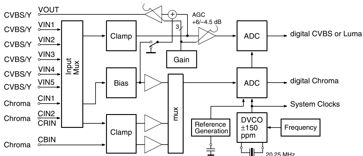
Fig. 2–1: Video front-end
