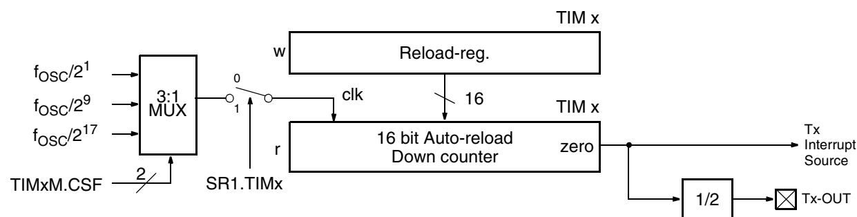
Fig. 5–22: Block diagram of timer T0 and T1
