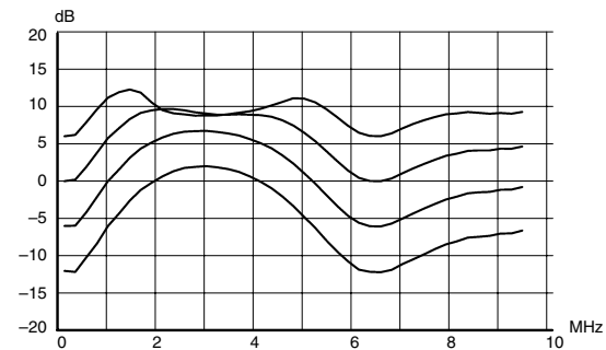
Fig. 2-13: Dynamic peaking frequency response
