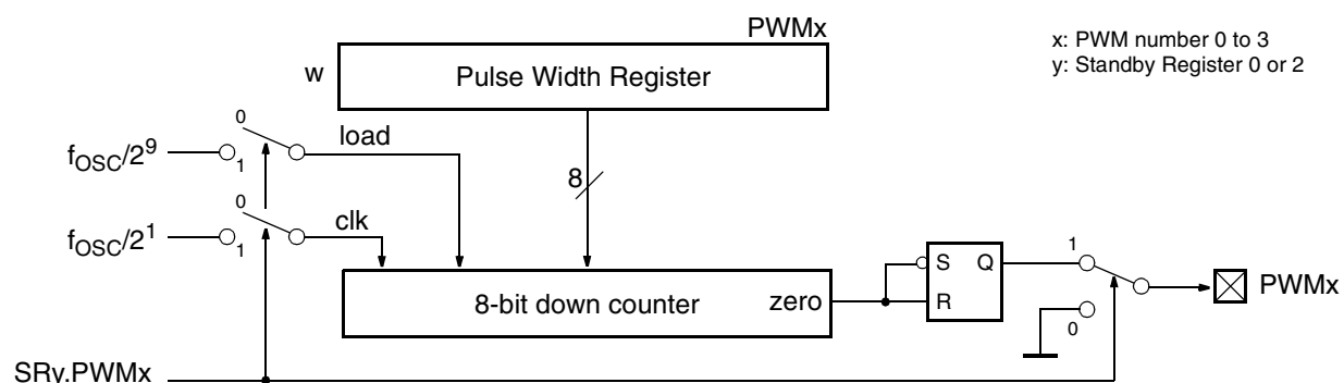
Fig. 5–24: Block diagram of 8-bit PWM
