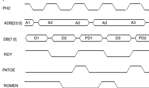
Fig. 5–17: Patch timing
