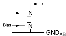
Fig. 6–15: Output pins ROUT, GOUT, BOUT, SVMOUT
