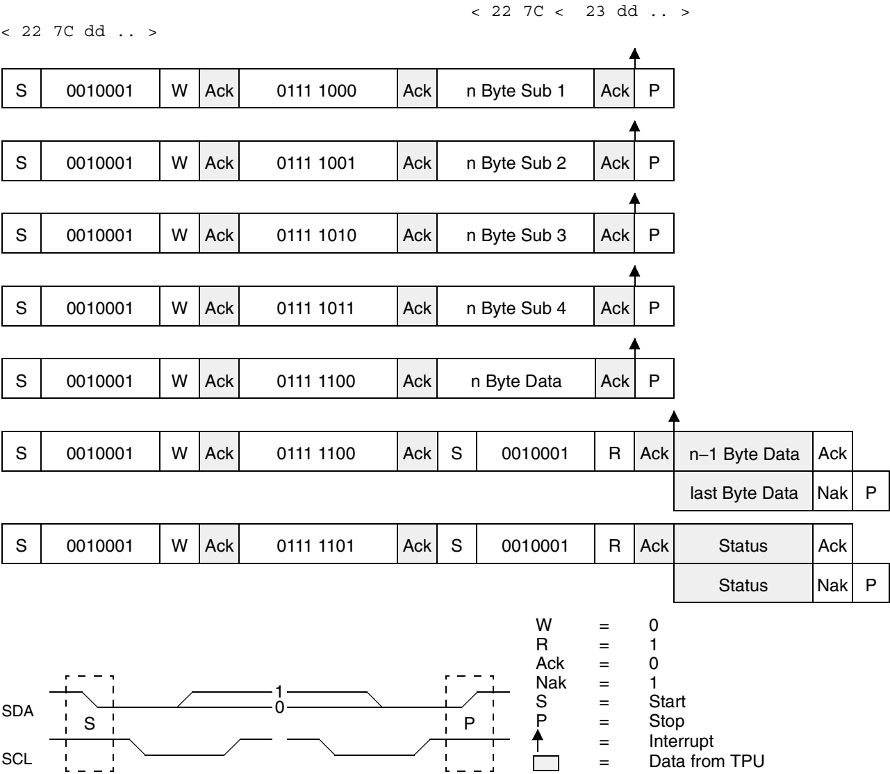
Fig. 3–23: I 2 C bus protocol
