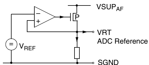
Fig. 6-13: Supply pins VRT, SGND
