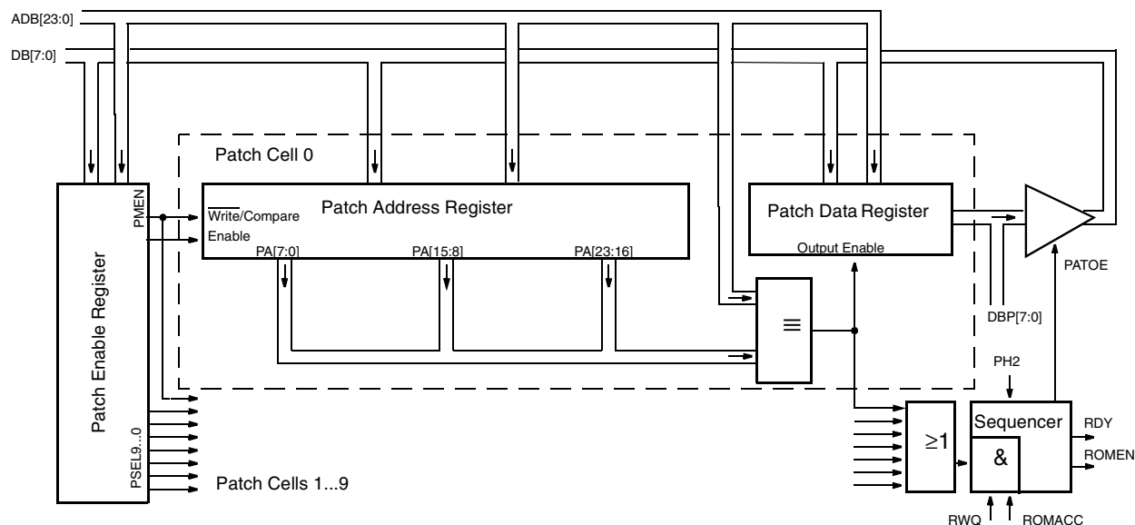
Fig. 5–16: Block diagram of patch module
