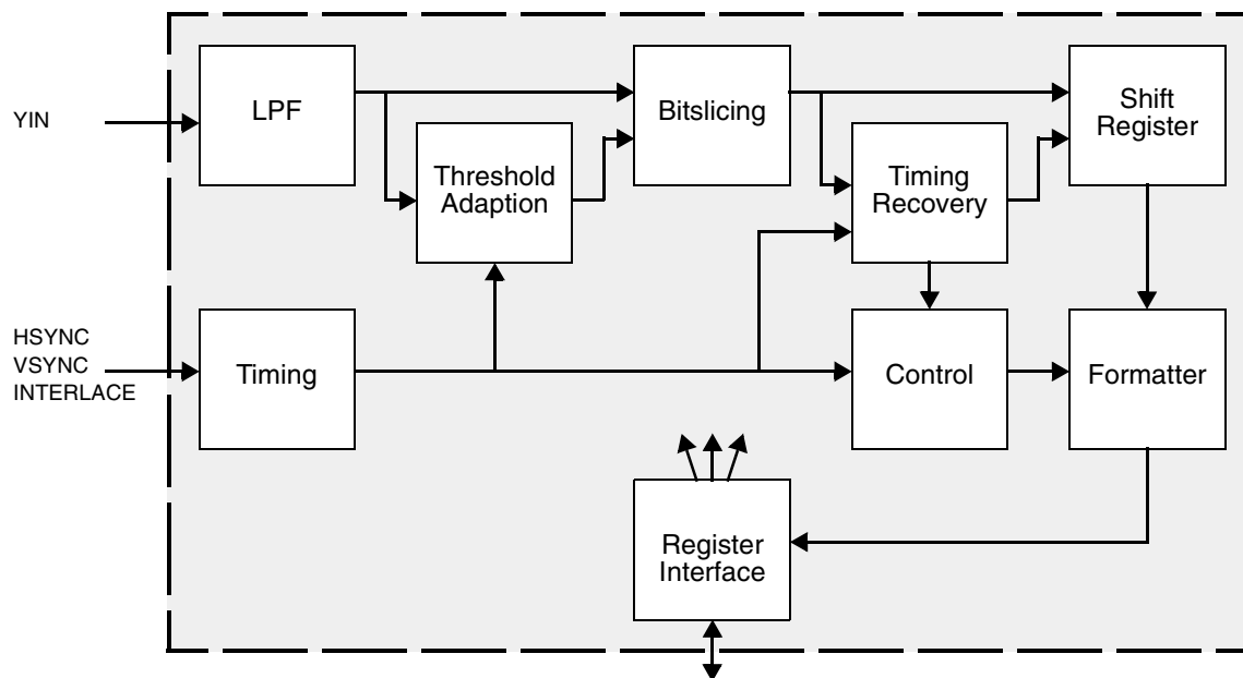
Fig. 5–28: Block diagram of Closed Caption Module
