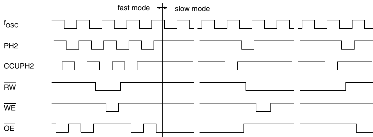
Fig. 5–1: Memory access signals
