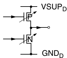
Fig. 6-8: Output pin CLK20
