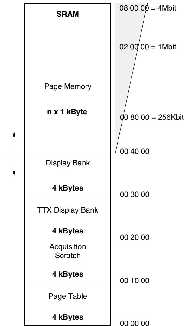
Fig. 3–4: Memory organization
