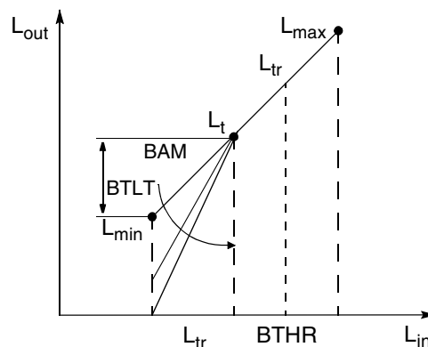
Fig. 2-11: Characteristics of the black-level expander
