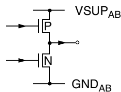
Fig. 6–19: Output pin INTLC
