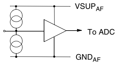
Fig. 6-11: Input pins CRIN, CBIN
