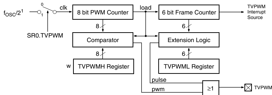
Fig. 5–26: Block Diagram of 14bit Tuning Voltage PWM
