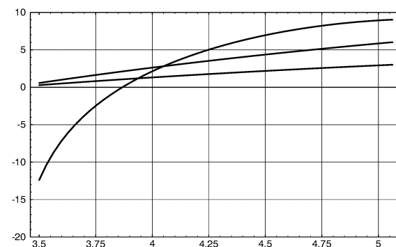
Fig. 2–3: Frequency response of chroma IF-compensation
