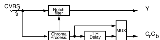
Fig. 2–8: SECAM color decoding
