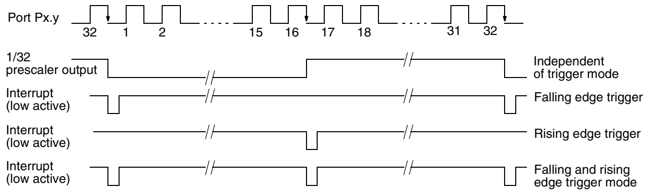
Fig. 5-14: Interrupt timing (1/32 Prescaler On)
