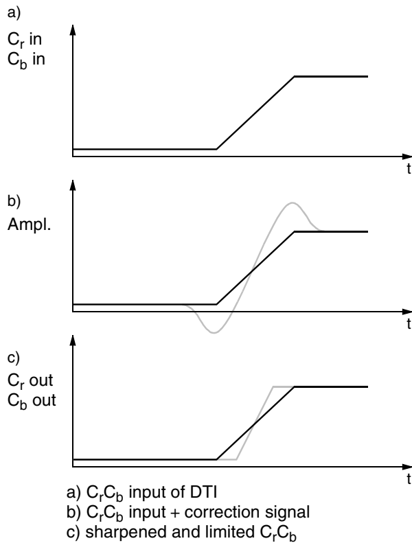
Fig. 2-16: Digital color transient improvement
