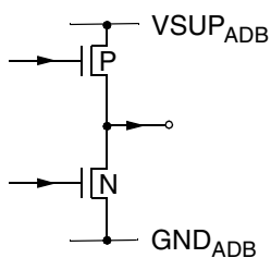
Fig. 6–29: Output pins ADB0-ADB18, \overline{\text{OE1}} , \overline{\text{OE2}} , WE1, WE2
