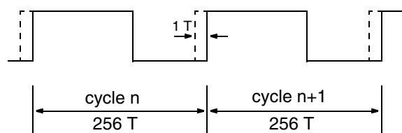
Fig. 5–25: TVPWM Timing
