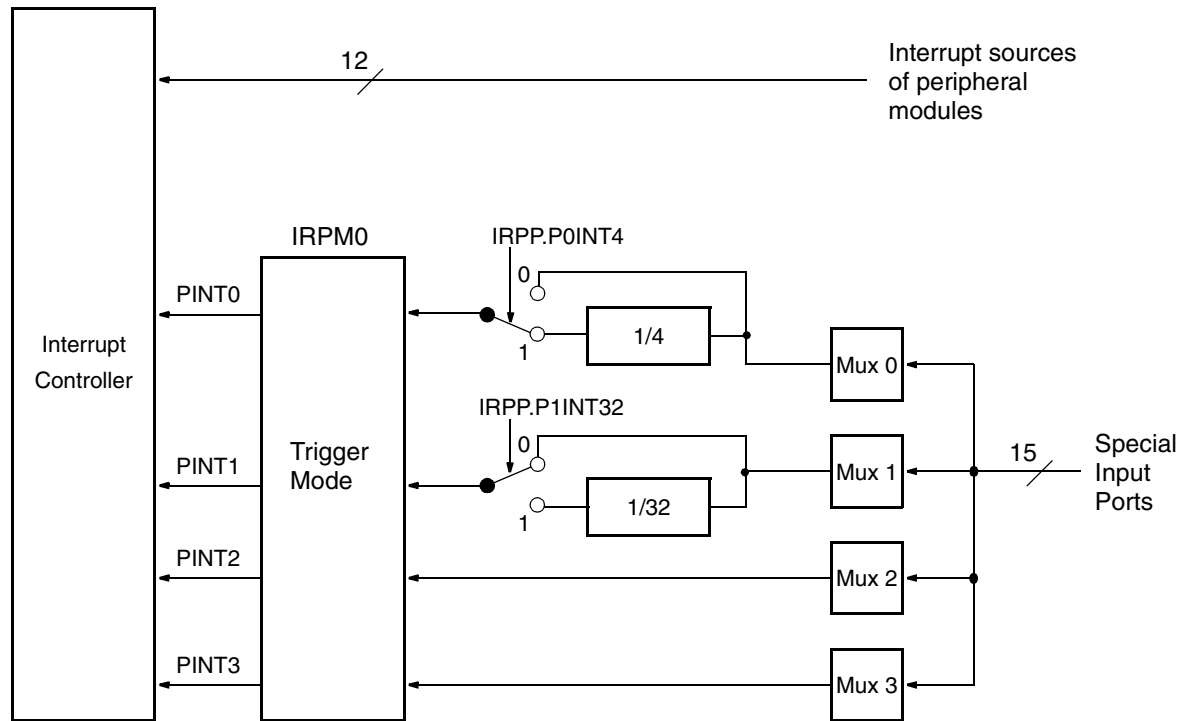
Fig. 5–12: Interrupt assignment and multiplexer
