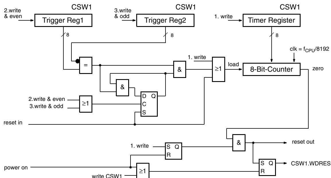
Fig. 5–4: Block diagram of watchdog
