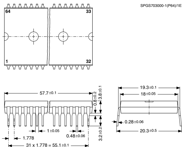
Fig. 6-1: 64-Pin Plastic Shrink Dual-Inline Package (PSDIP64)
