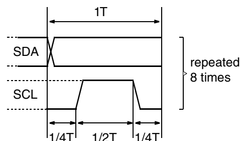
Fig. 5–20: Single bit on I²C bus
