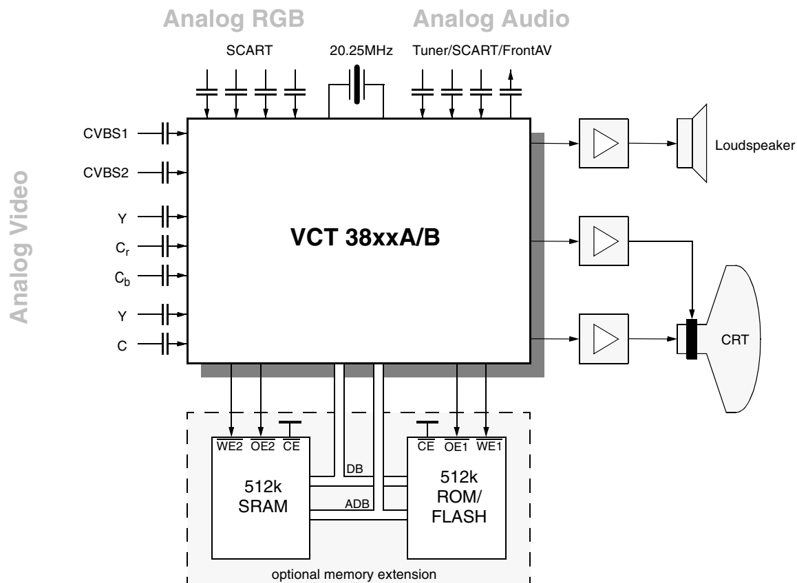
Fig. 1–3: Single-chip TV with VCT 38xxA/B
