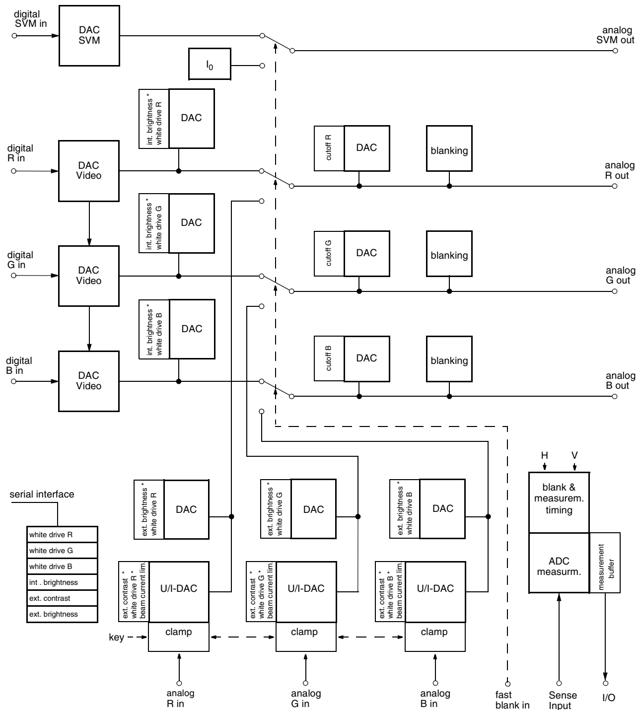
Fig. 2–23: Video back-end
