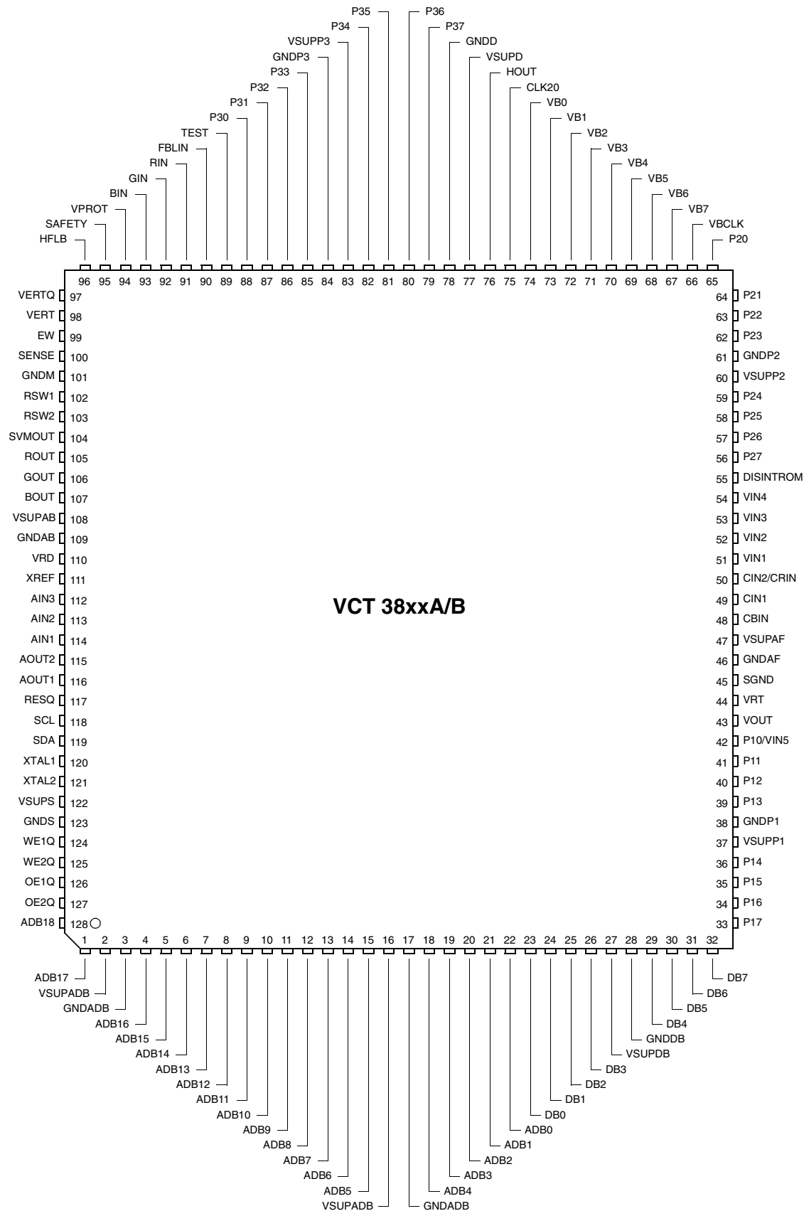
Fig. 6–4: PMQFP128 package
