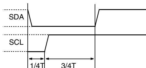
Fig. 5–21: Stop condition I²C bus
