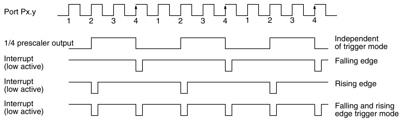
Fig. 5-13: Interrupt timing (1/4 Prescaler On)
