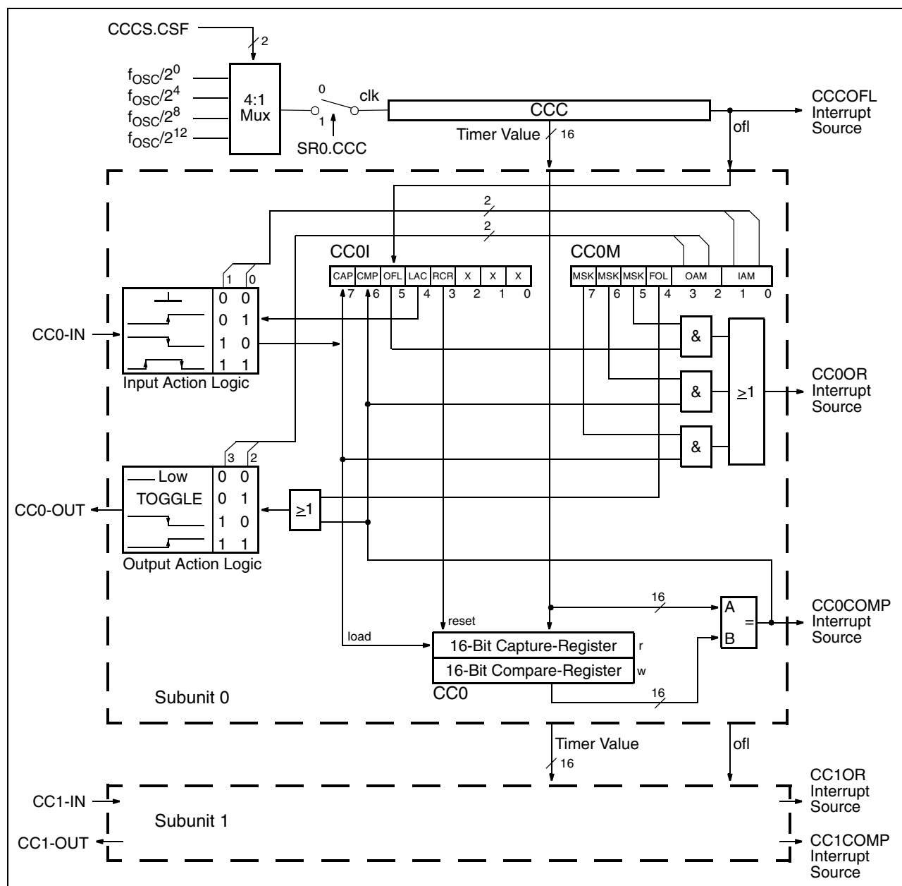
Fig. 5-23: Block diagram of CAPCOM module
