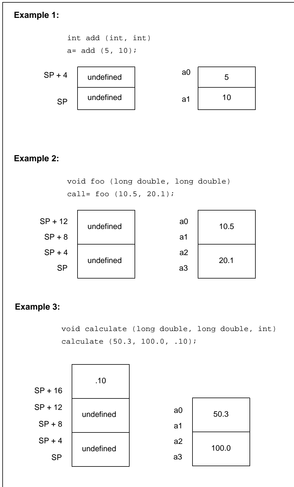
FIGURE 10-1: PASSING ARGUMENTS
