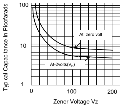
Figure 1 Capacitance vs. V_Z Curve
