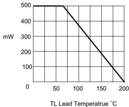
Figure 2 - Derating Curve
