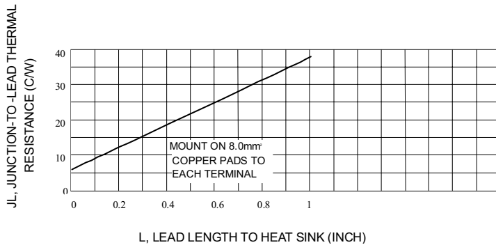
Fig. 4-TYPICAL THERMAL RESISTANCE
